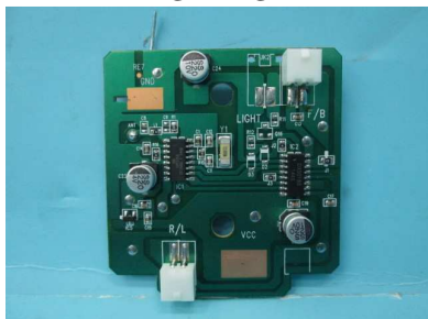
Inner Circuit Top View of model GF4MS
