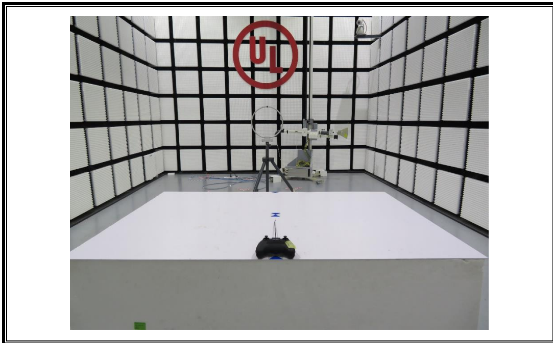
RADIATED RF MEASUREMENT SETUP (Below 30MHz– X axis)
