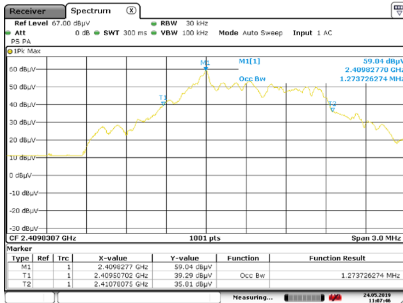
99% OCCUPIED BANDWIDTH LOW CH
