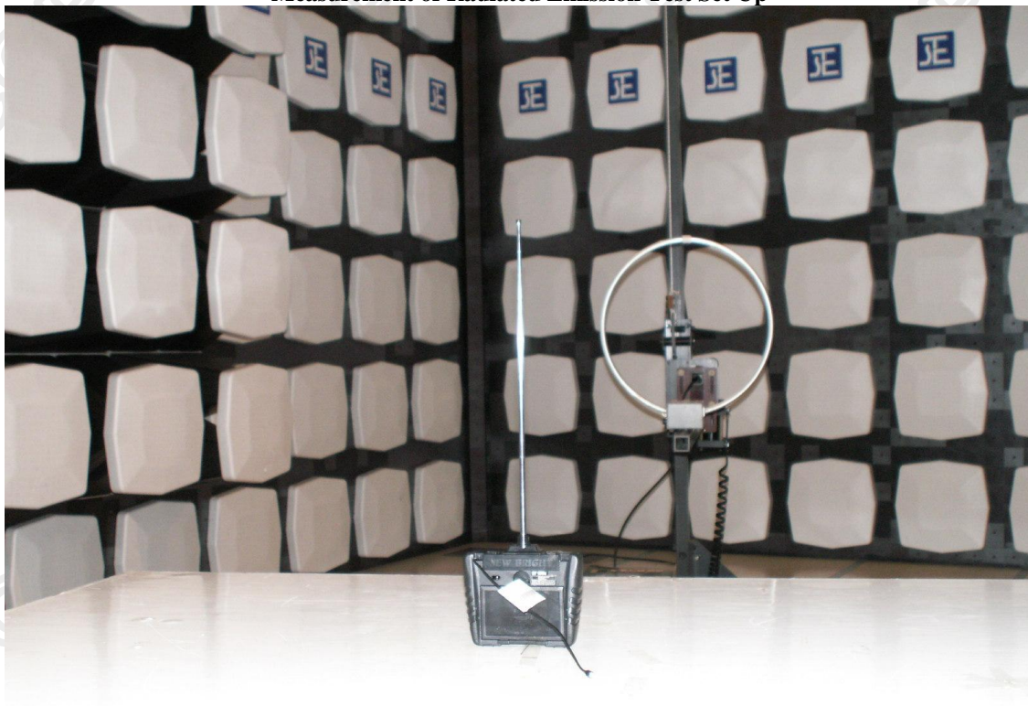
Measurement of Radiated Emission Test Set Up
