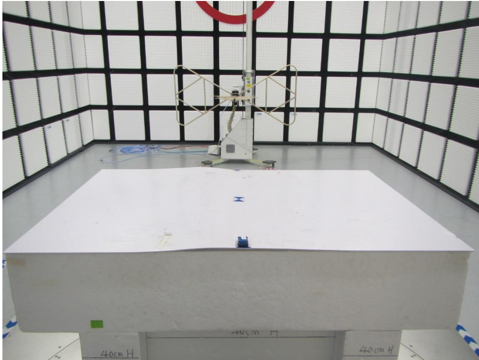
Radiated Disturbance Above 1G
