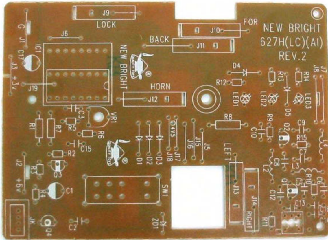
Model : 6277H(49M) Component side
