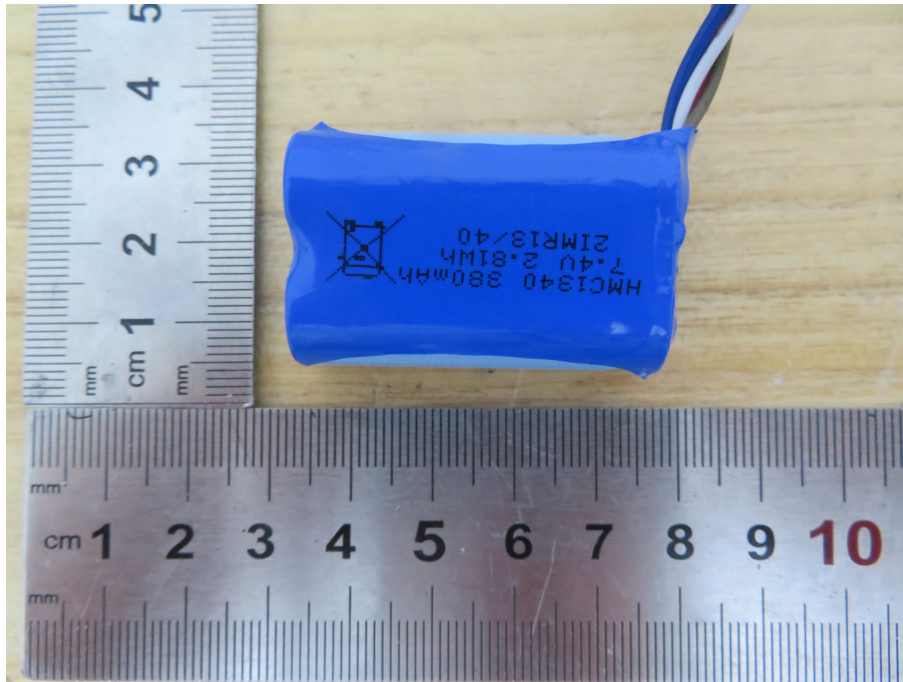
Internal View of EUT-6(380mAh)
