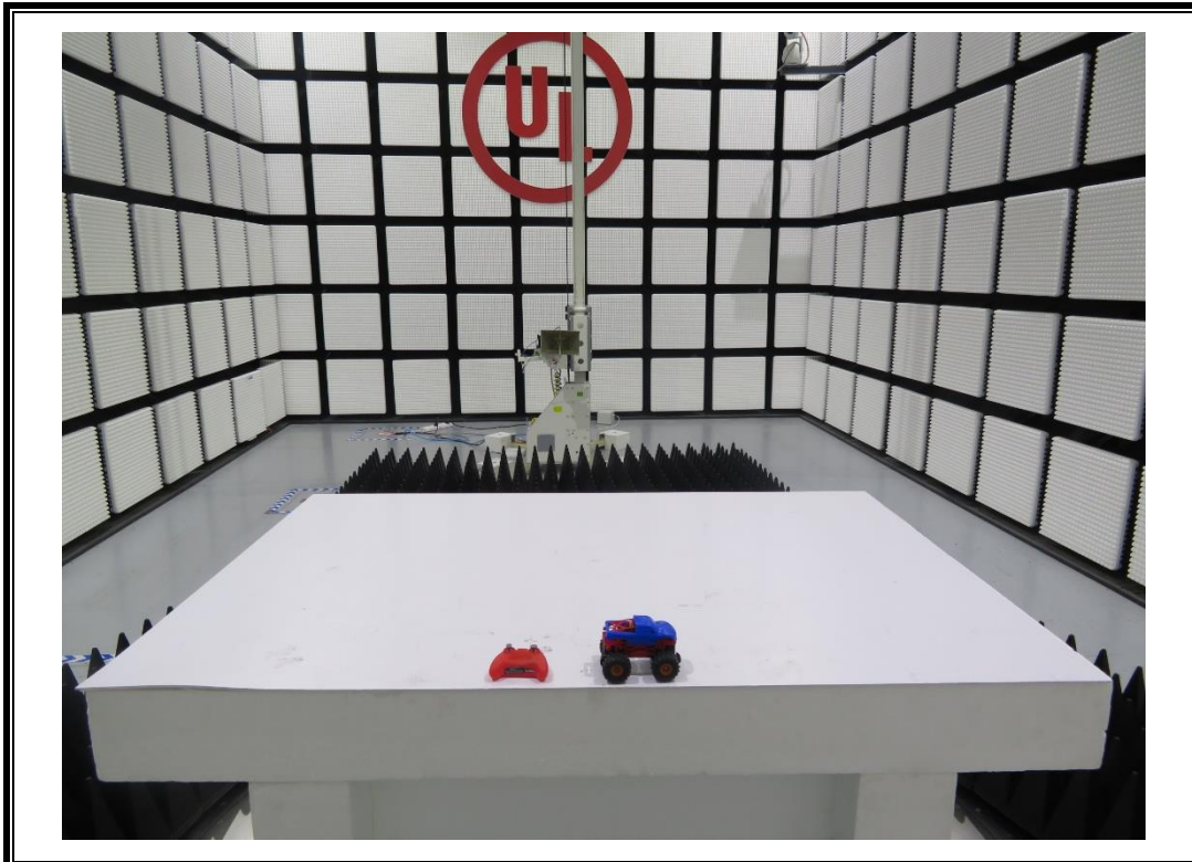
RADIATED RF MEASUREMENT SETUP (Above 1GHz)
