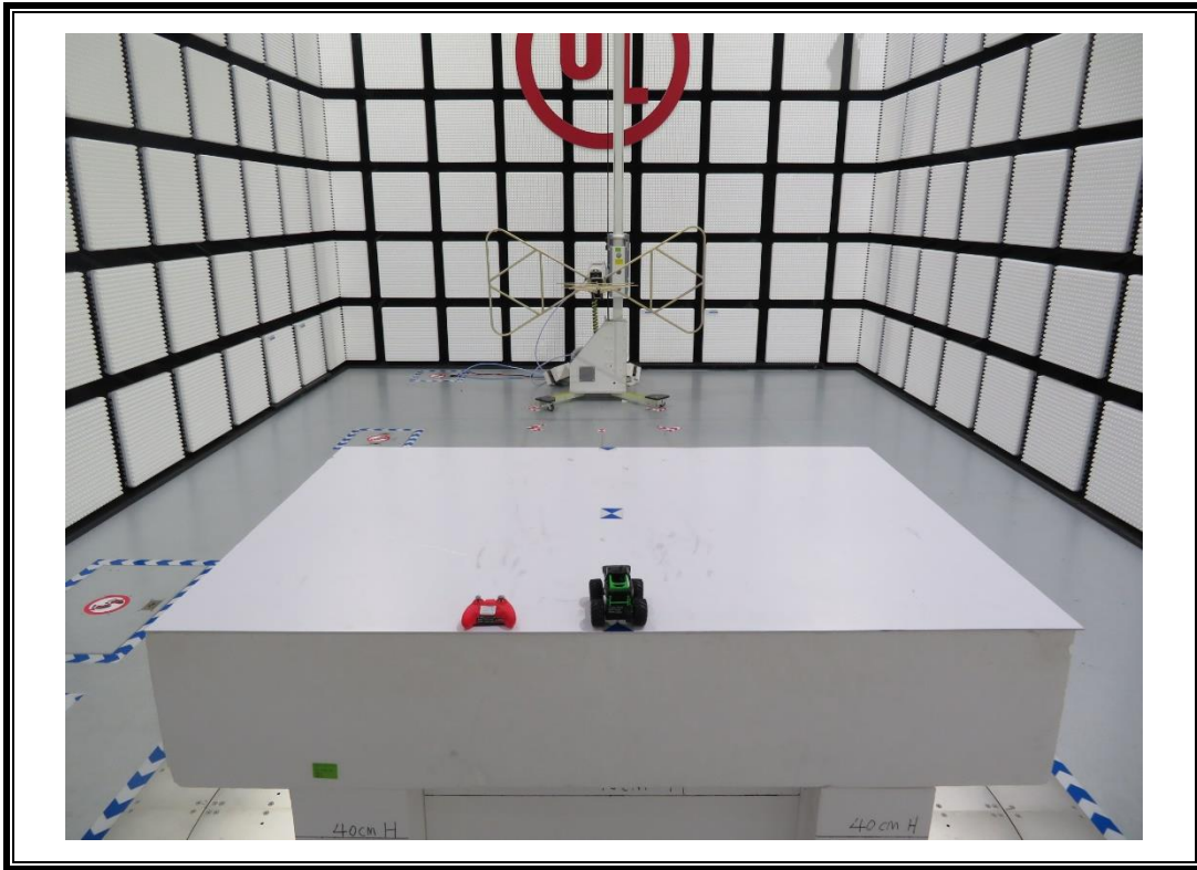
RADIATED RF MEASUREMENT SETUP (30MHz ~ 1 GHz)
