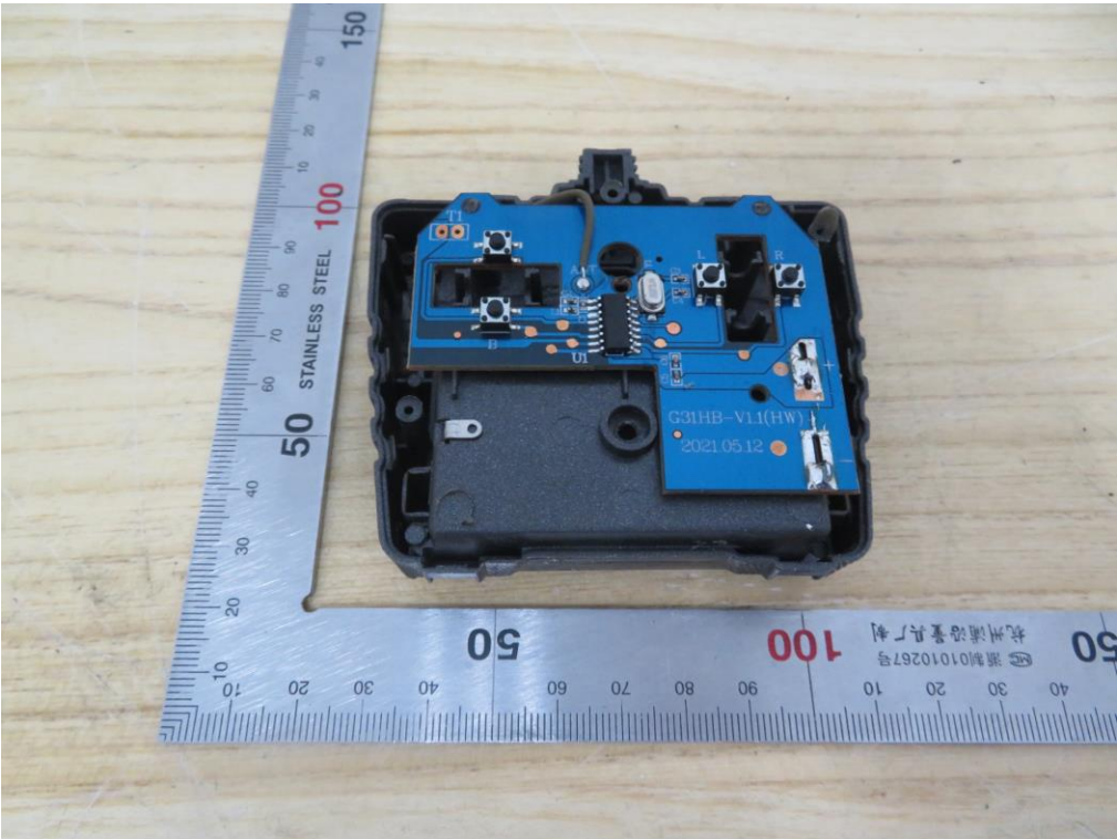
Internal View of EUT (Version 3)-3
