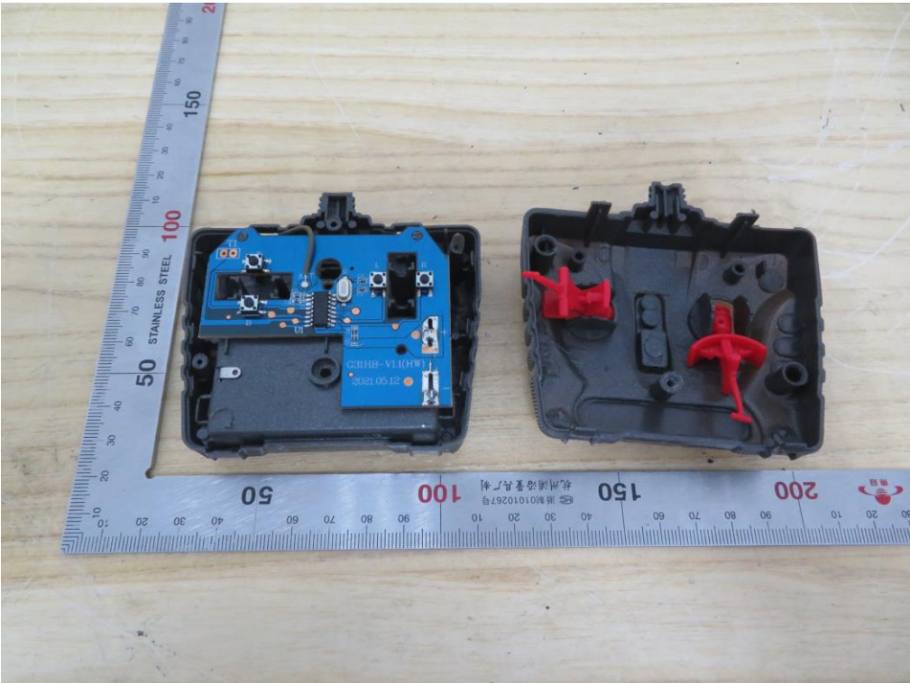
Internal View of EUT (Version 3)-2
