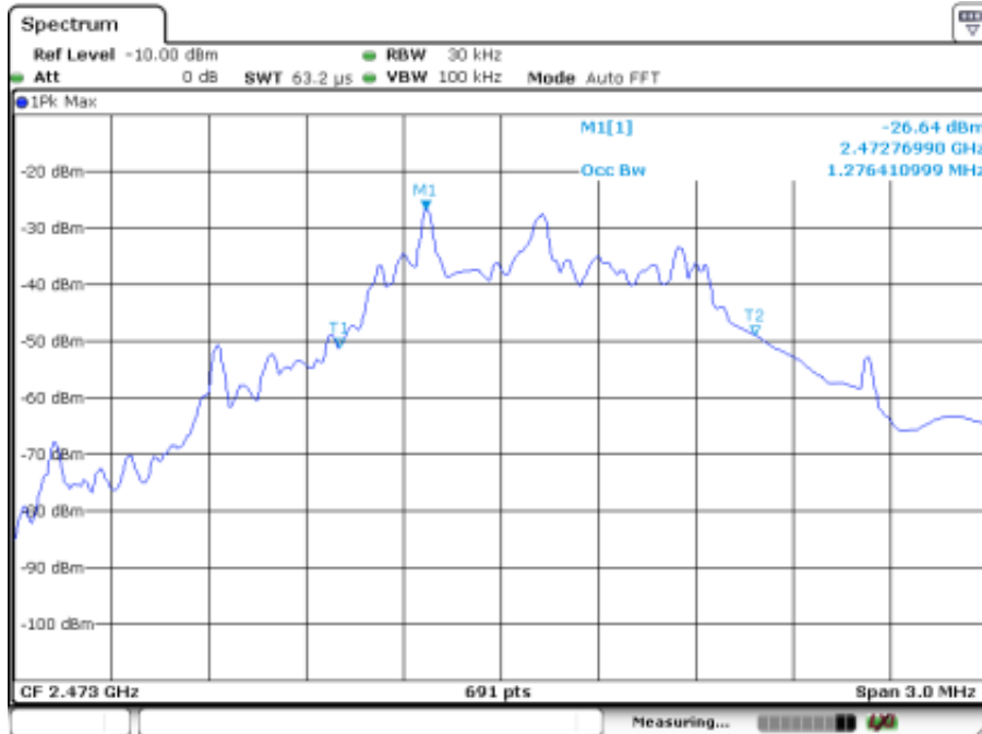
99% OCCUPIED BANDWIDTH HIG CH
