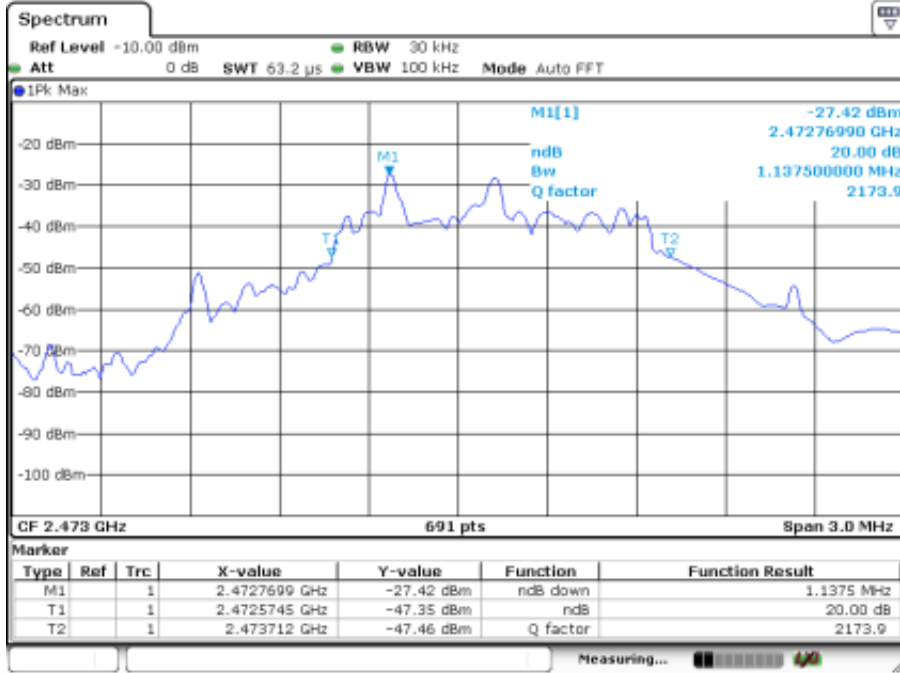
20 dB BANDWIDTH HIG CH
