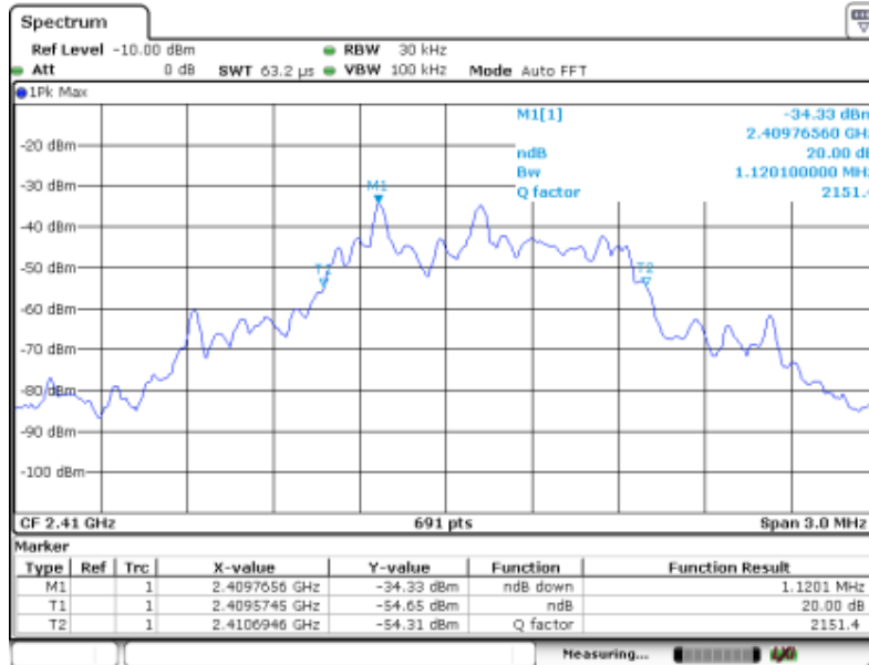
20 dB BANDWIDTH LOW CH
