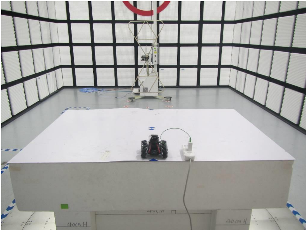
Radiated Emissions below 1GHz test setup photo Charging
