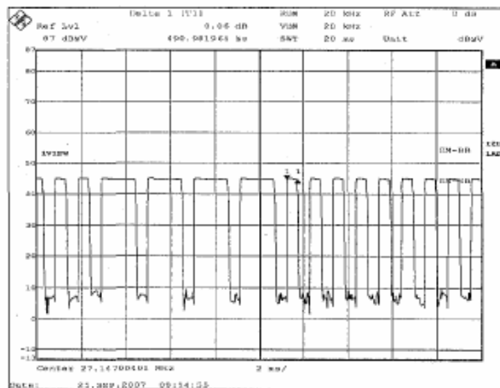
Figure C [Short Pulse]
