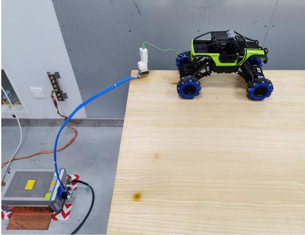
Radiated Disturbance Below 1GHz Charging
