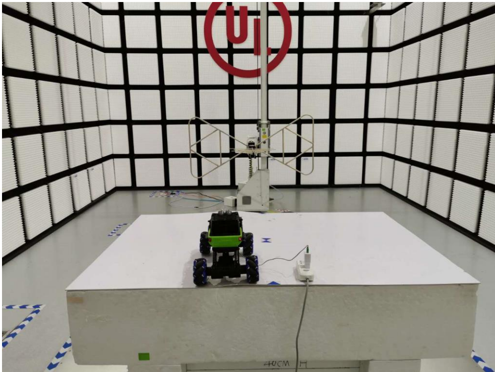
Radiated Disturbance Below 1GHz Charging
