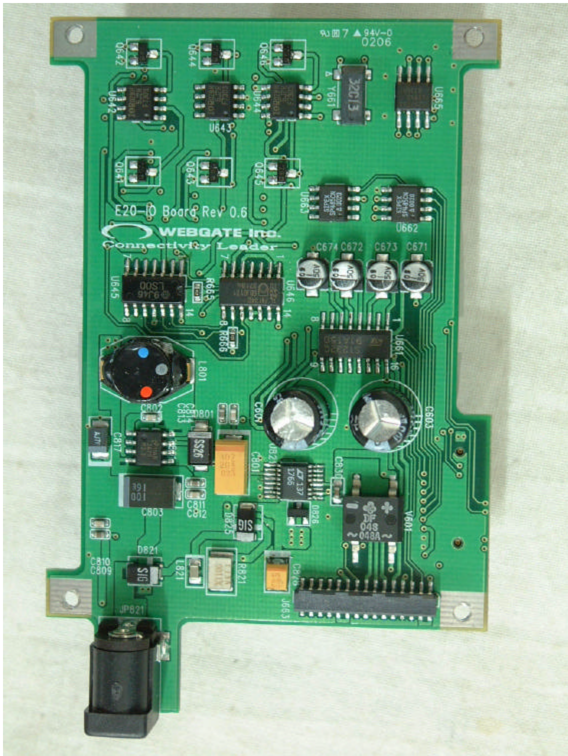
<FRONT VIEW OF E20-IO BOARD>
