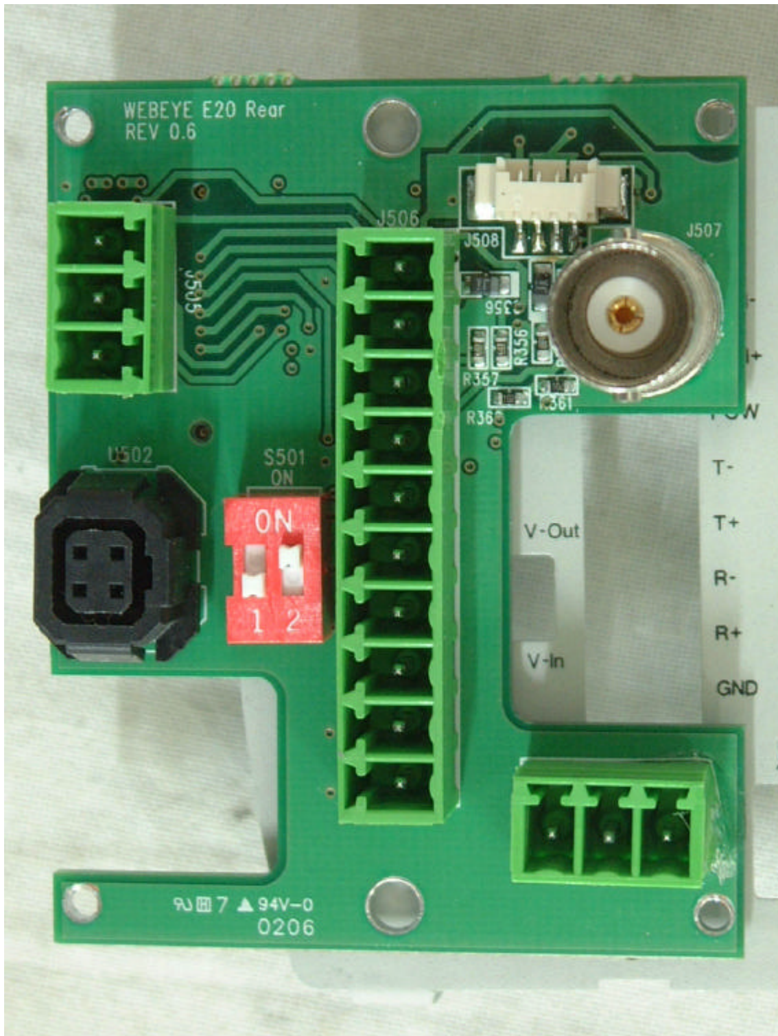
<FRONT VIEW OF CONNECTOR BOARD>
