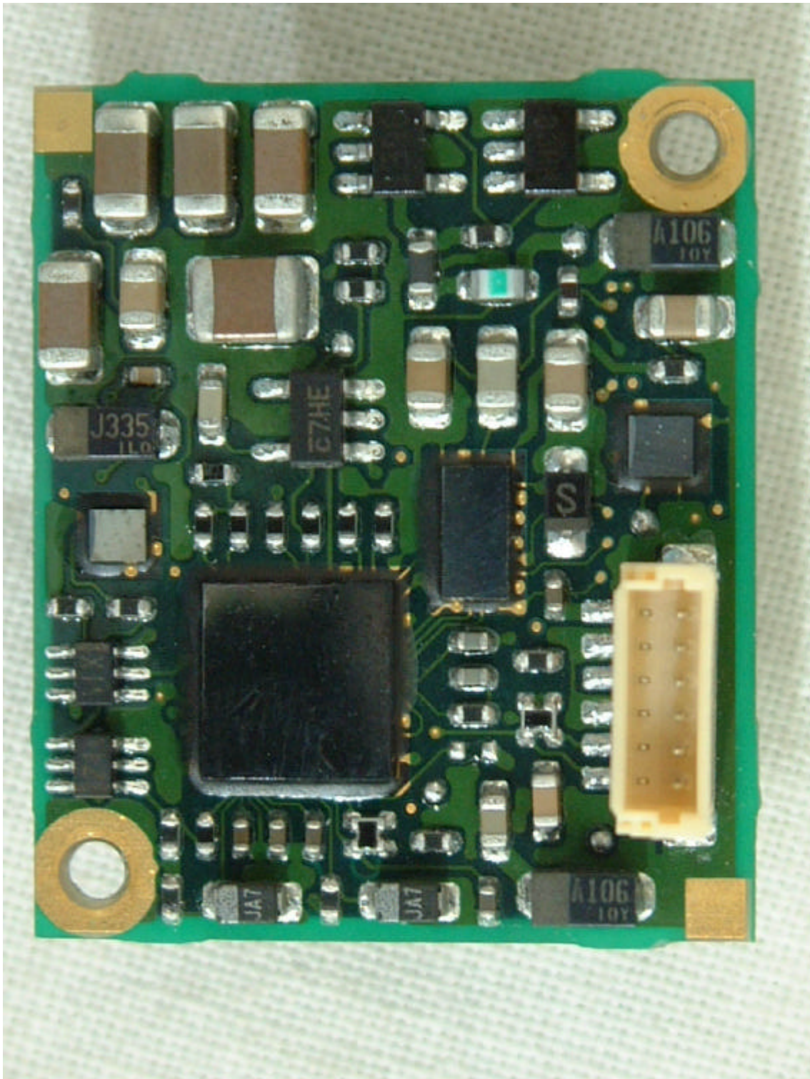
<REAR VIEW OF CAMERA BOARD>
