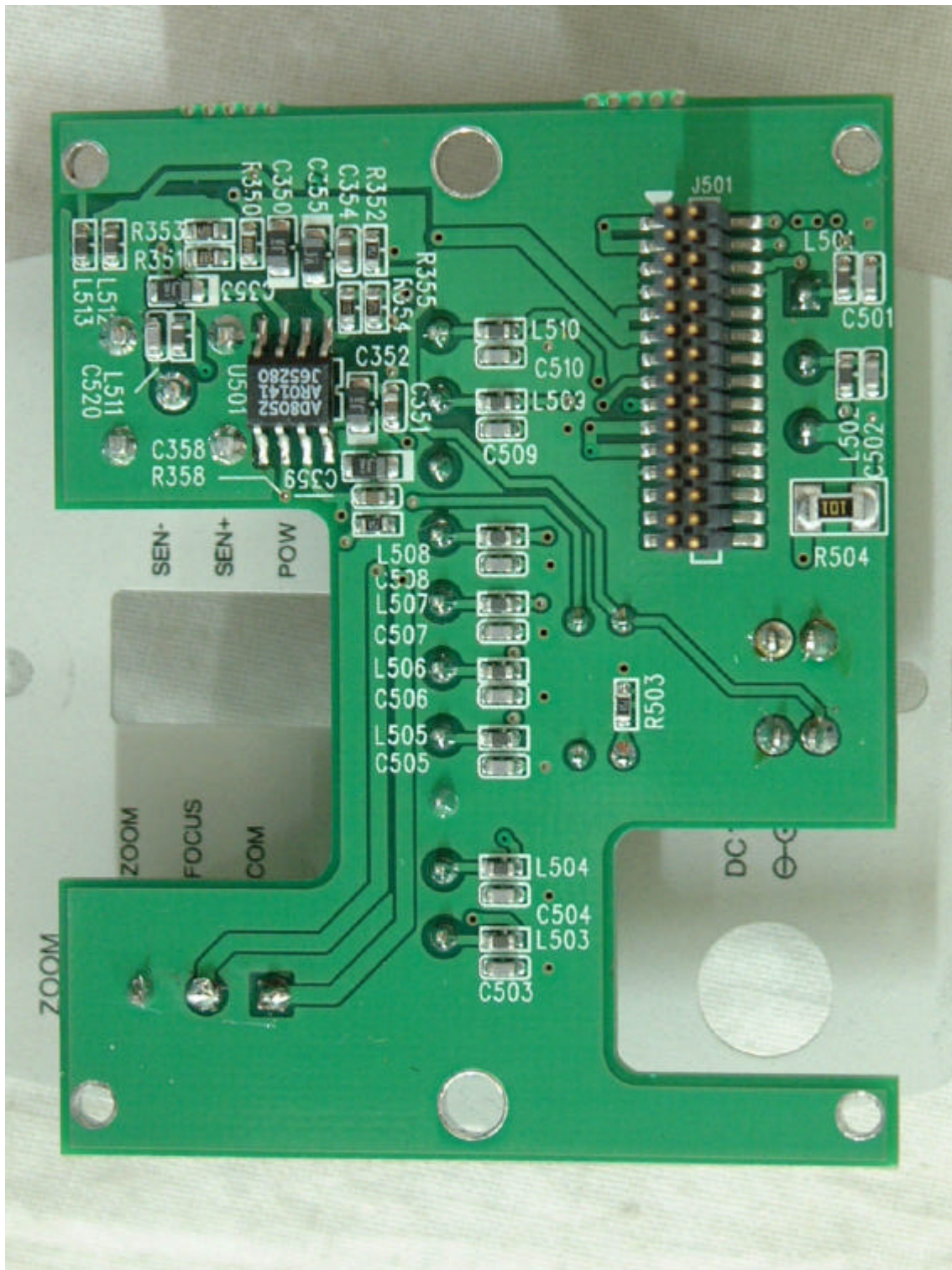
<REAR VIEW OF CONNECTOR BOARD>
