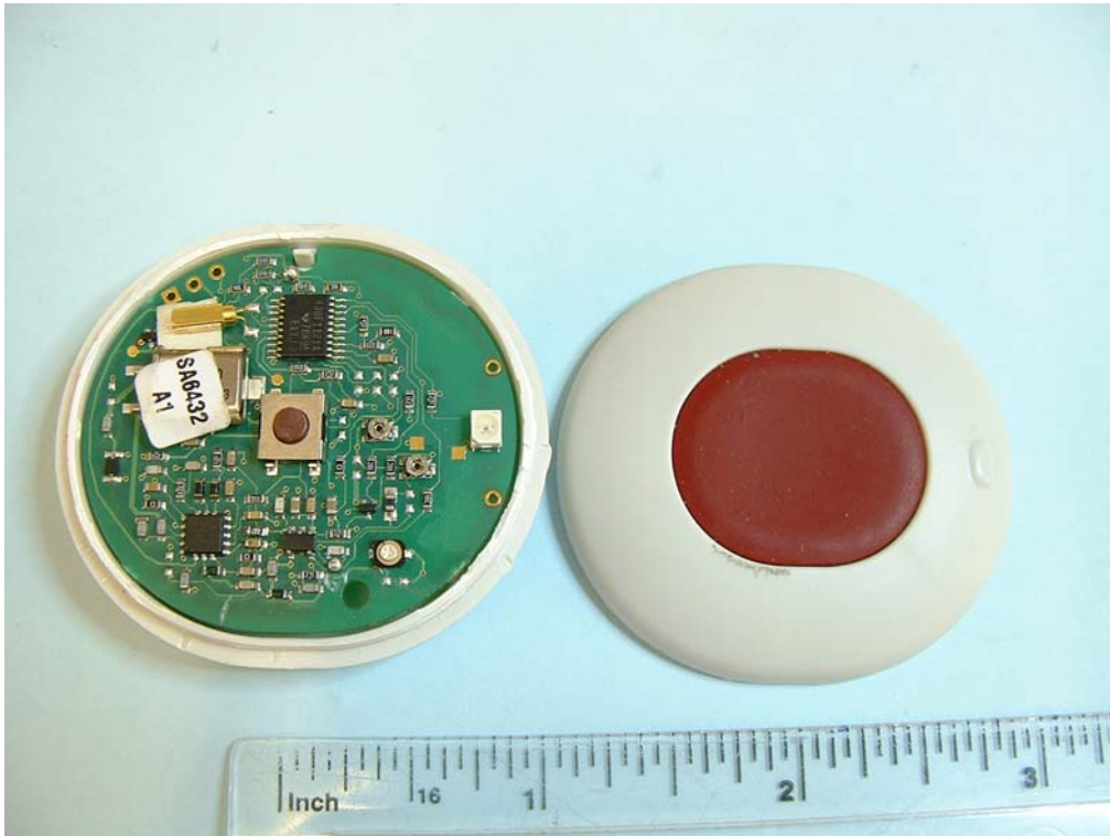
TOP VIEW CASE REMOVED
