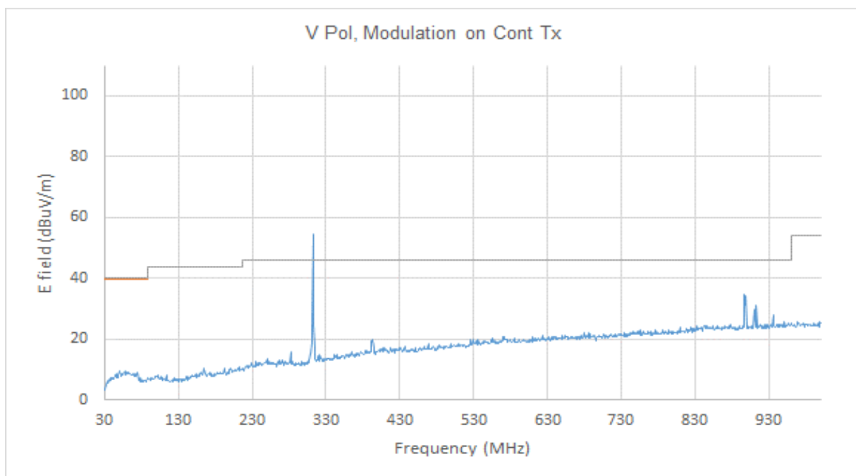
Figure 3: Electric field emissions Plot, 30MHz to 1GHz, Vertical
