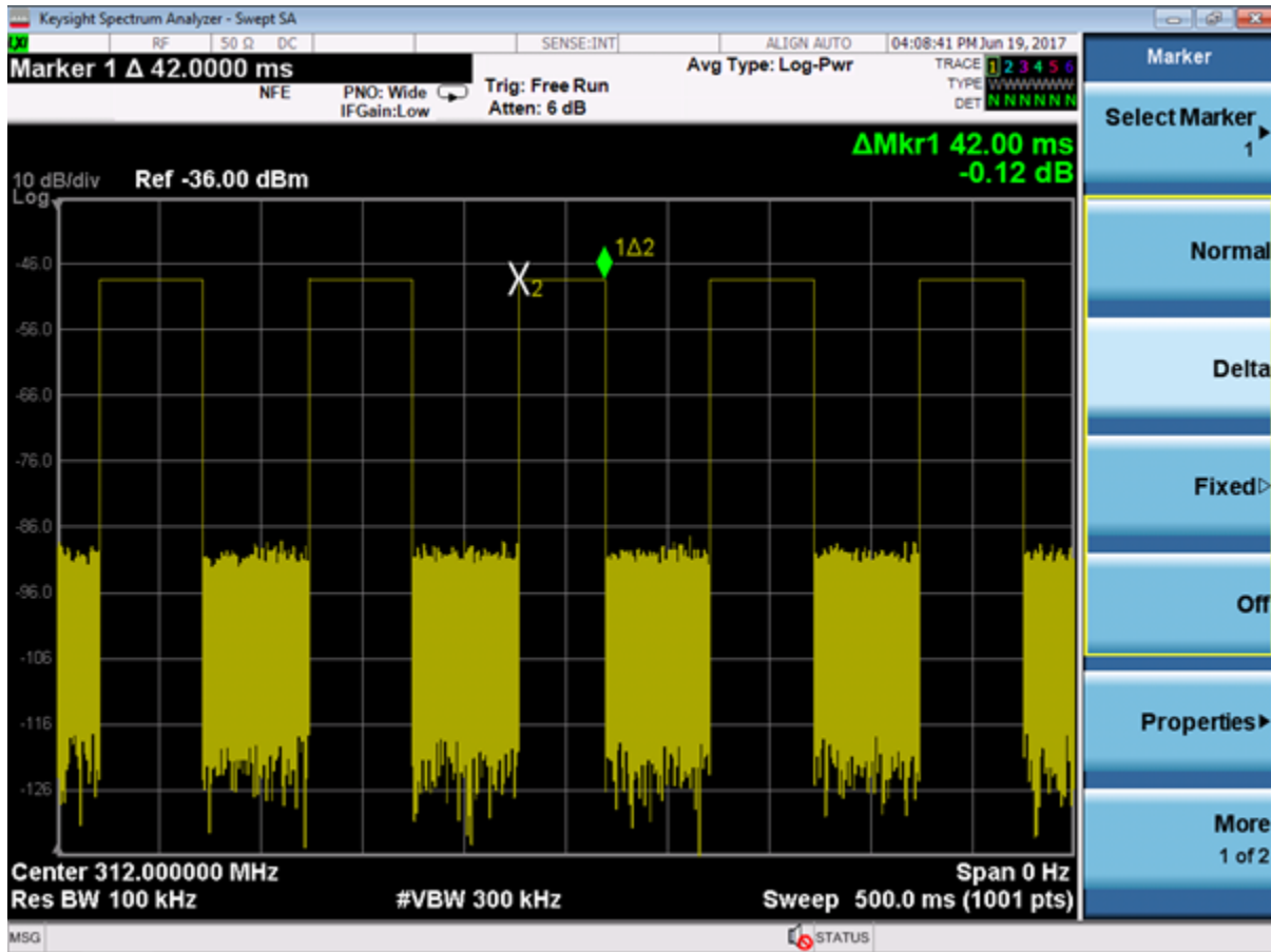
Figure 15 Measurement of pulse width t
