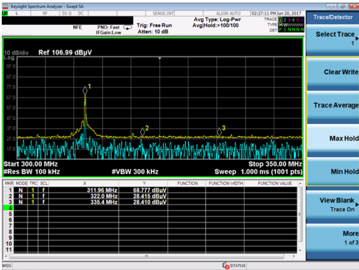
Figure 9 Upper restricted band measurement
