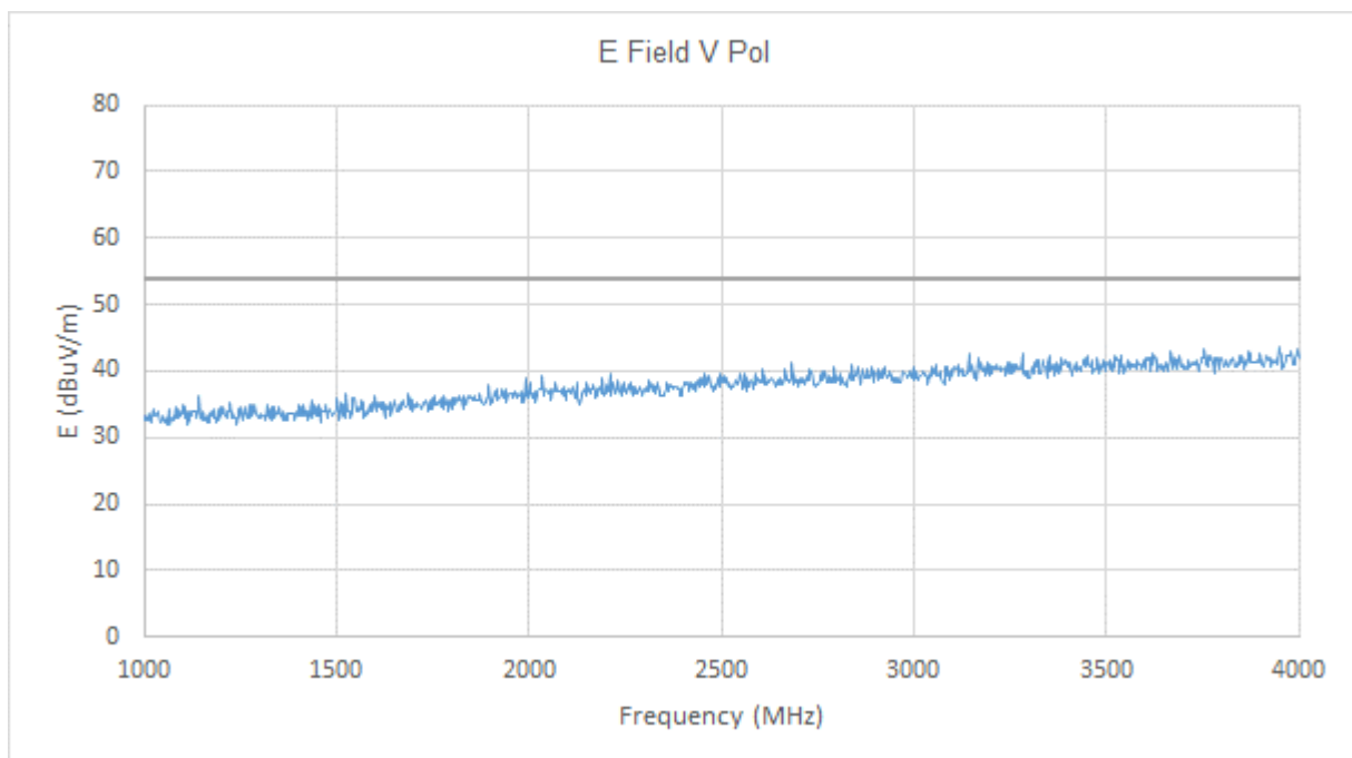
Figure 6: Electric field emissions Plot, 1GHz to 4GHz – Vertical Polarity
