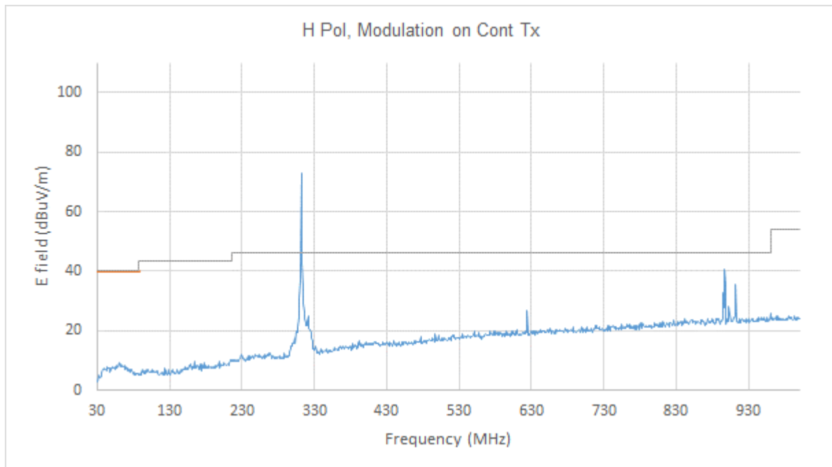
Figure 2: Electric field emissions Plot, 30MHz to 1GHz, Horizontal
