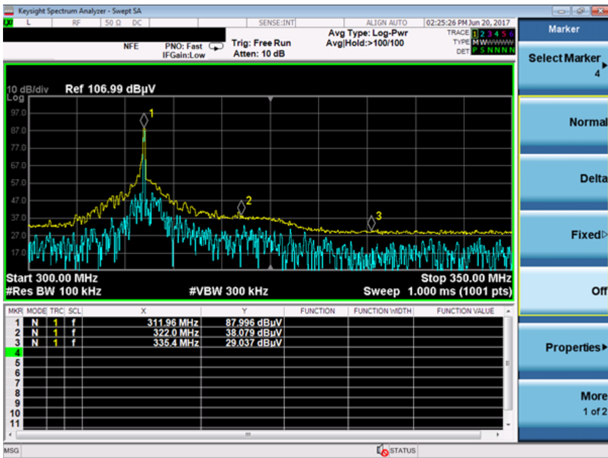
Figure 10 Upper restricted band measurement
