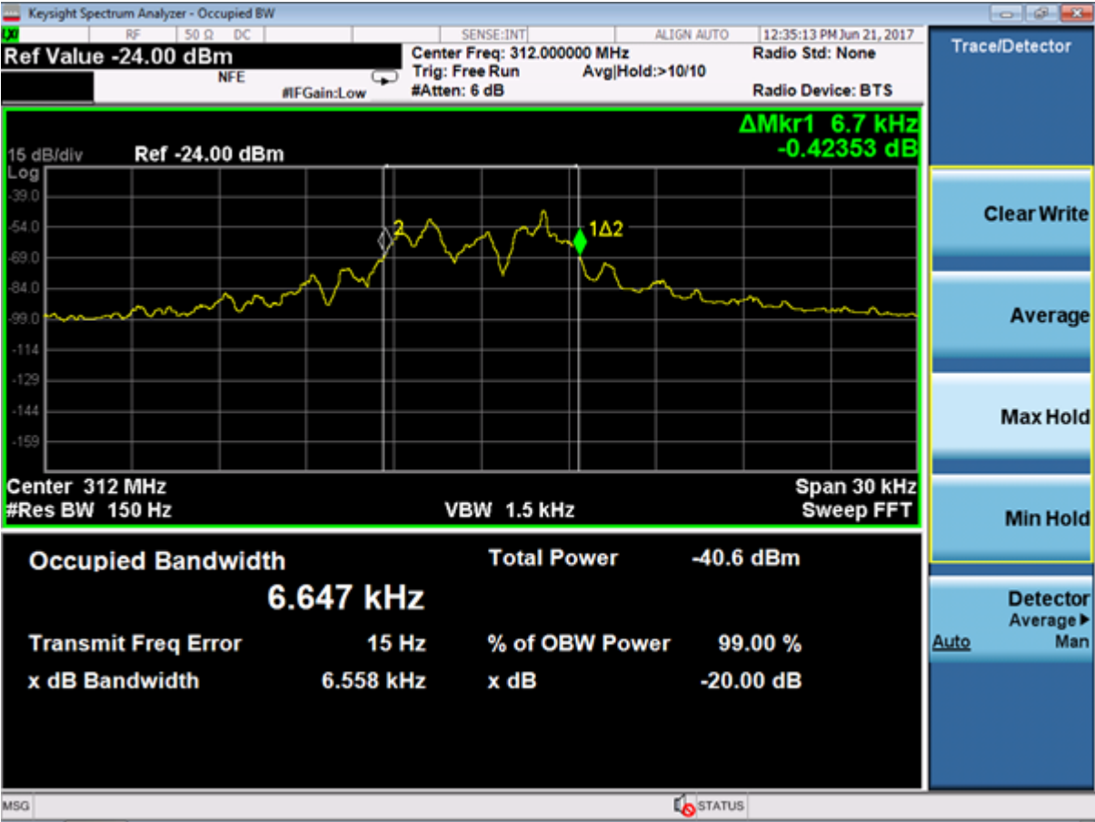
Figure 11 Bandwidth measurement horizontal polarity
