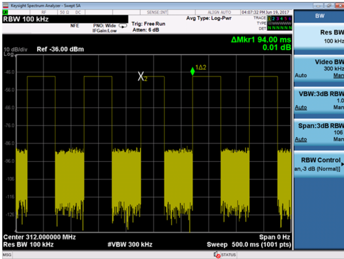
Figure 14 Measurement of pulse width T
