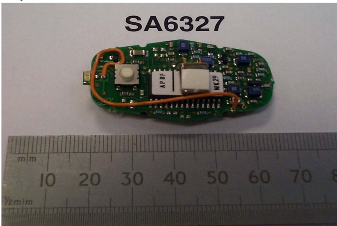
Component side
