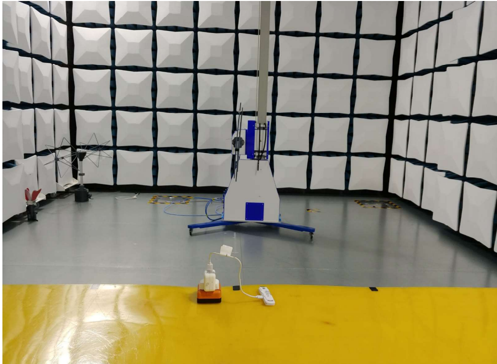
Set-up for Radiated Emission Above 1GHz
