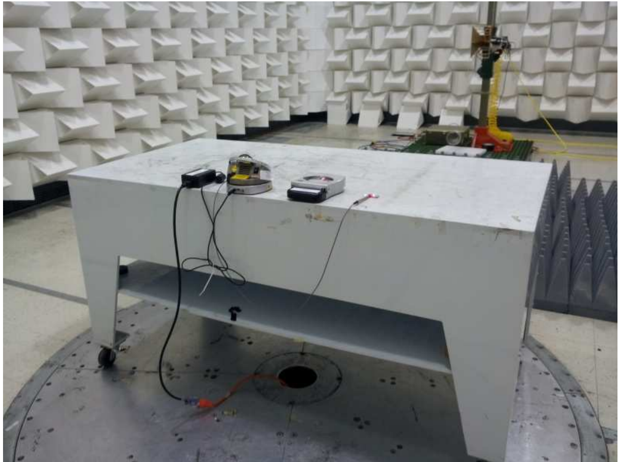
Rear view
