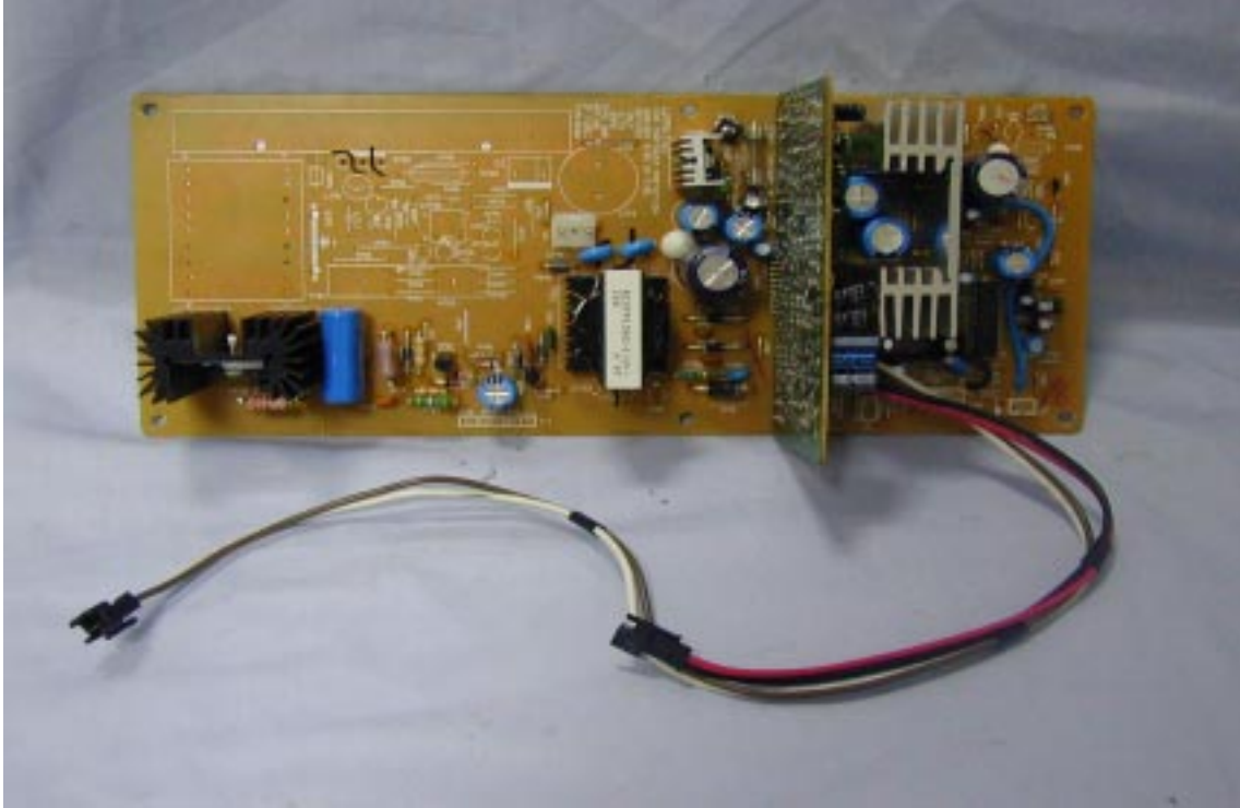
Component Side View of Audio Amplifier
