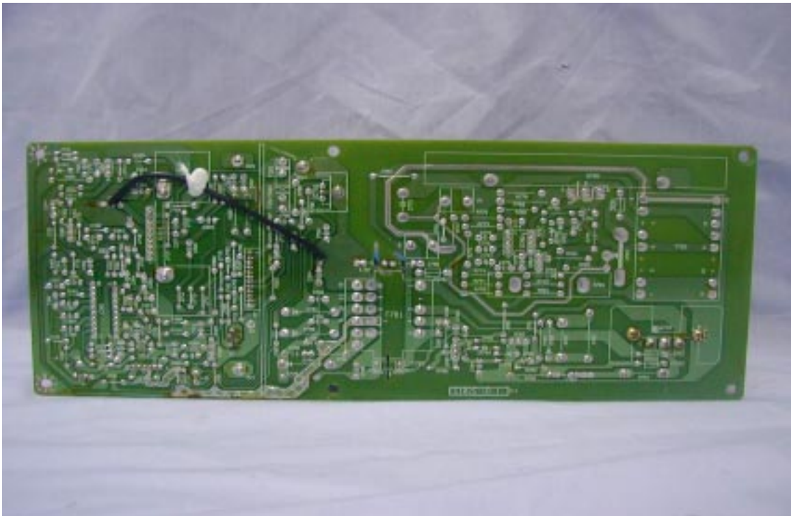
Solder Side View of Audio Amplifier
