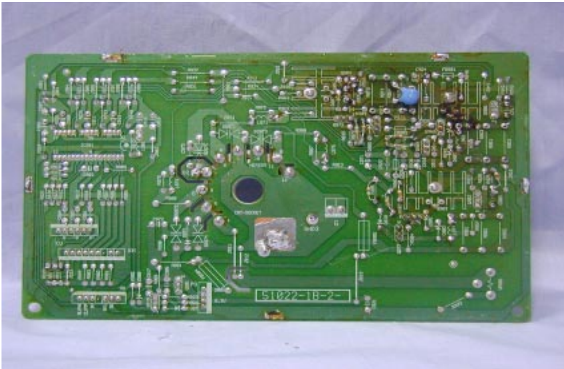
Solder Side View of CRT Board
