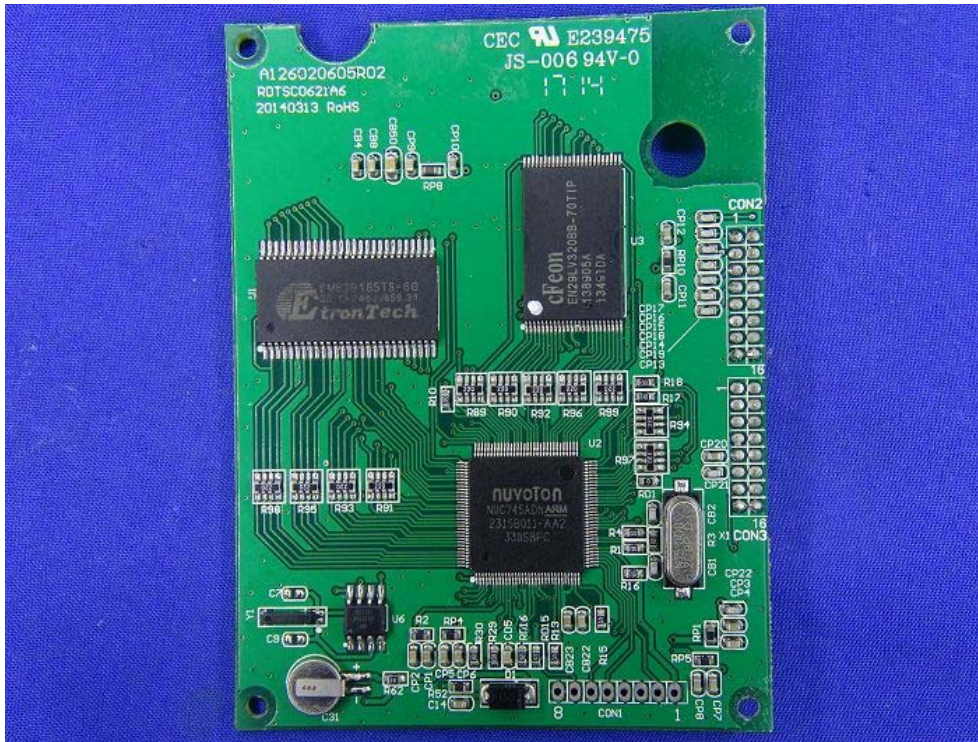
(22) EUT Photo
