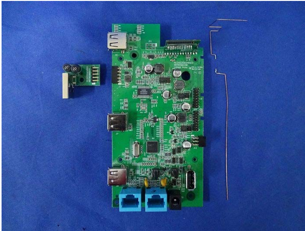
(25) EUT Photo
