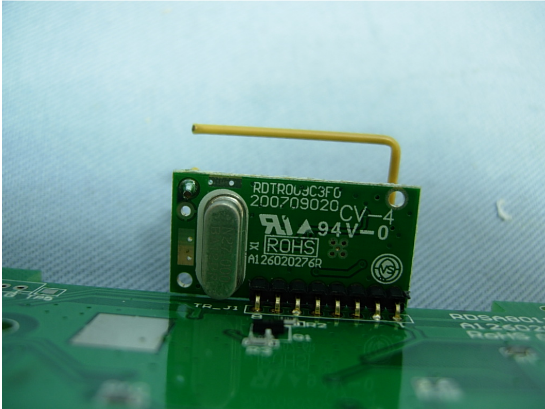
(15) EUT Photo (RF Modular with curve antenna)
