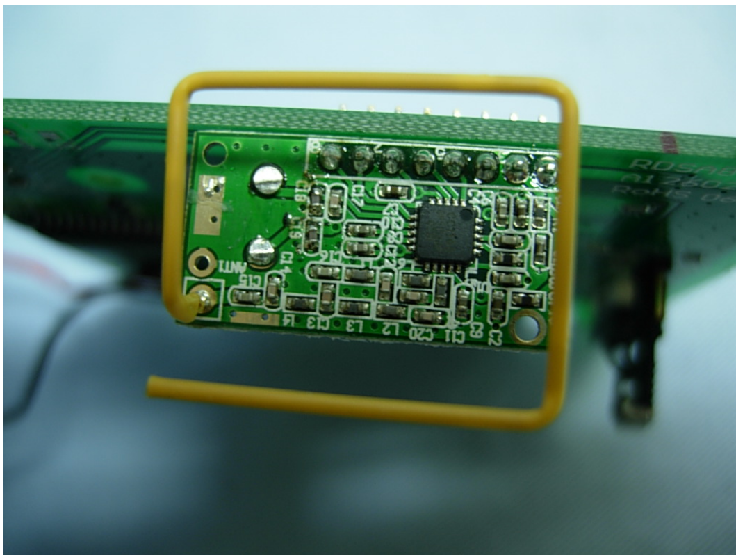
(14) EUT Photo (RF Modular with curve antenna)
