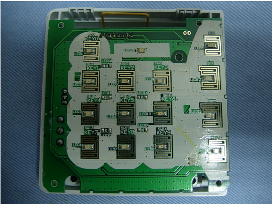
(20) EUT Photo (M/N: SA801-2)
