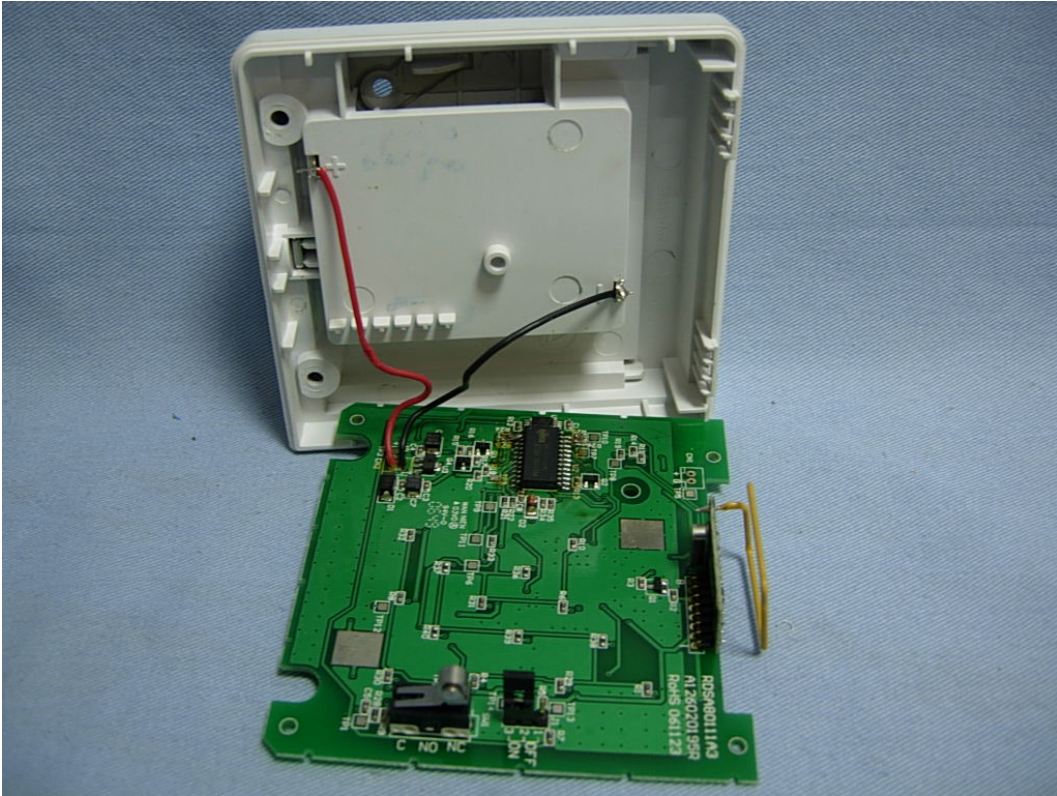
(21) EUT Photo (M/N: SA801-2)
