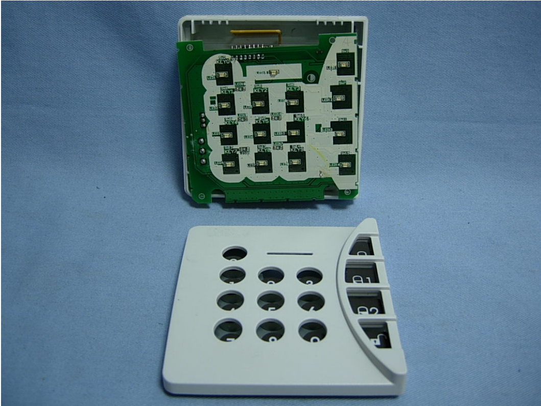
(19) EUT Photo (M/N: SA801-2)
