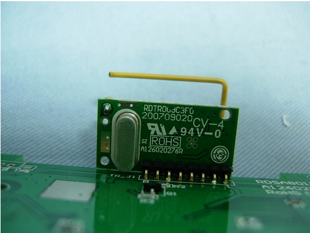
(4) EUT Photo (RF Modular with curve antenna)
