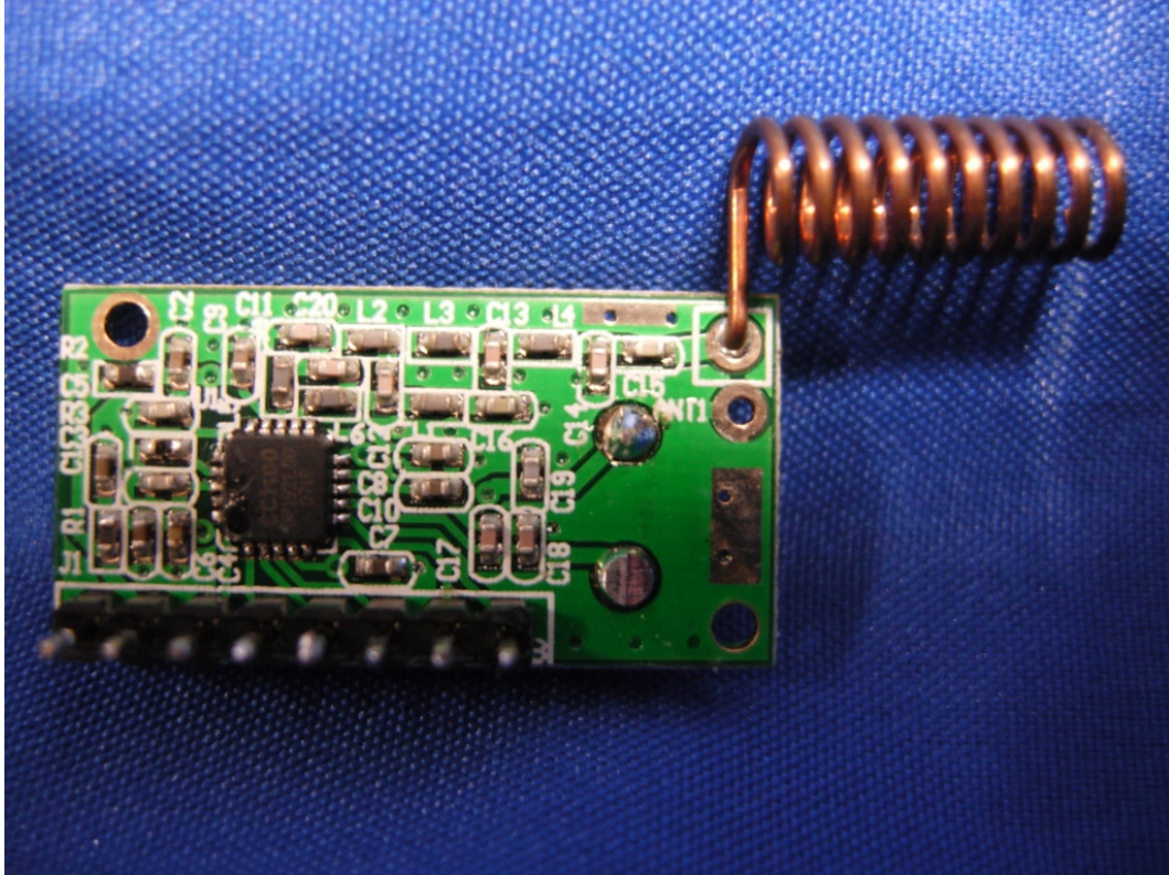
(1) EUT Photo (RF Modular with winding antenna)
