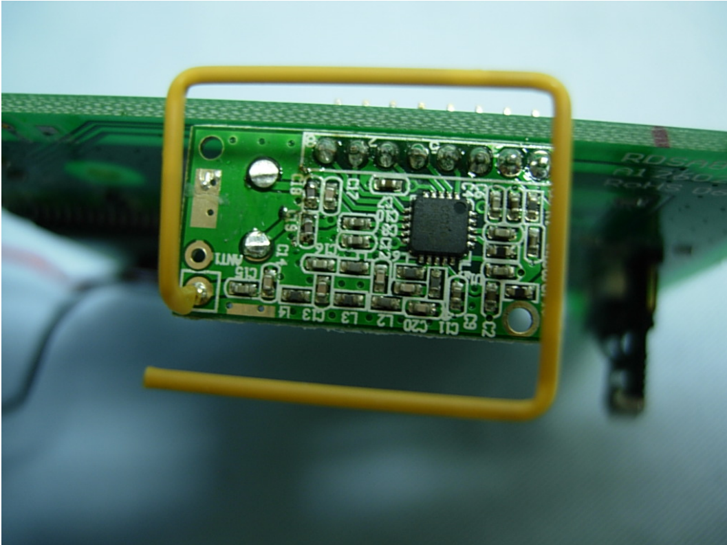
(3) EUT Photo (RF Modular with curve antenna)
