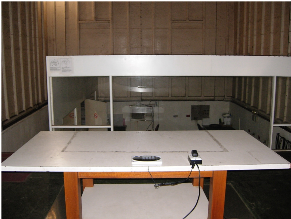
Back View of Radiated Test (Horn) (Mode 1)
