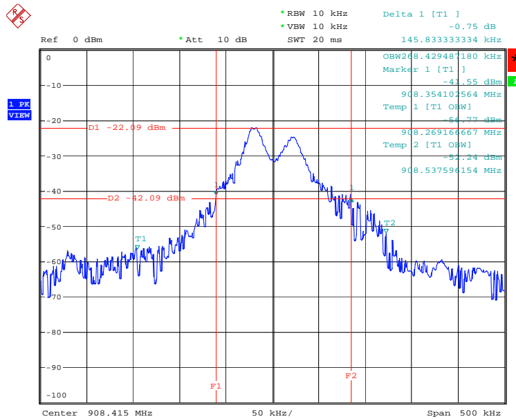
20 dB/99% Bandwidth Plot on 908.42 MHz
