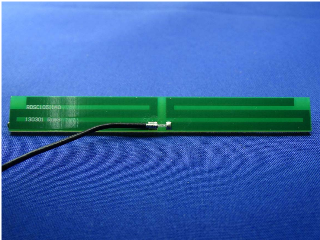
(28) EUT Photo -Antenna
