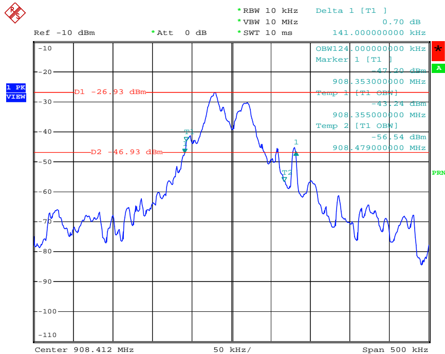
20 dB/99% Bandwidth Plot on 908.42 MHz
