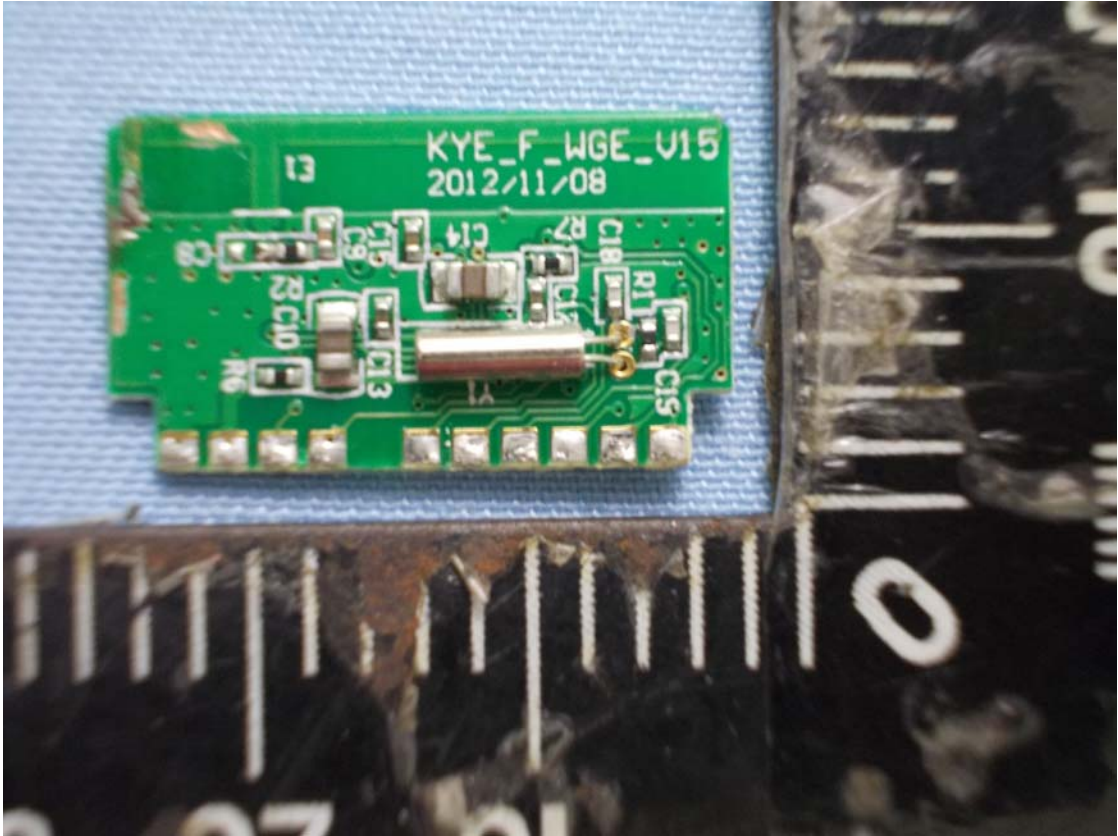
13 Rear view of PCB 1
