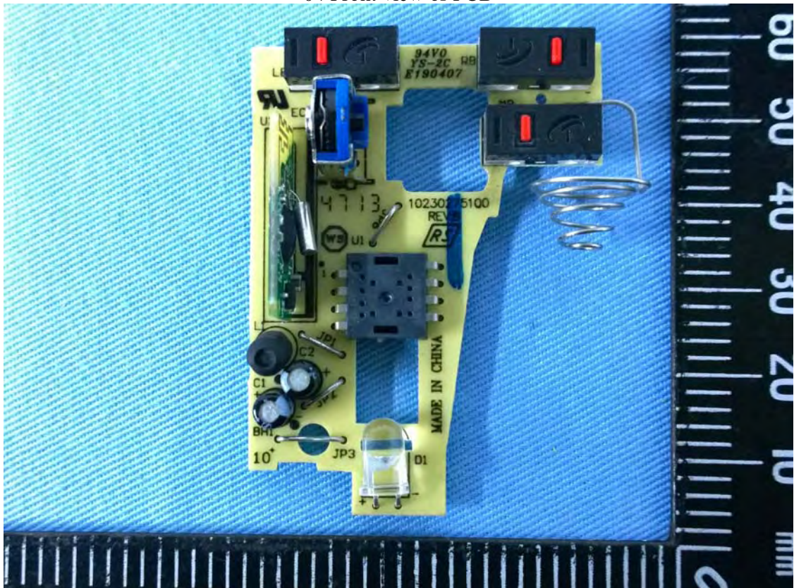
04 Front view of PCB
