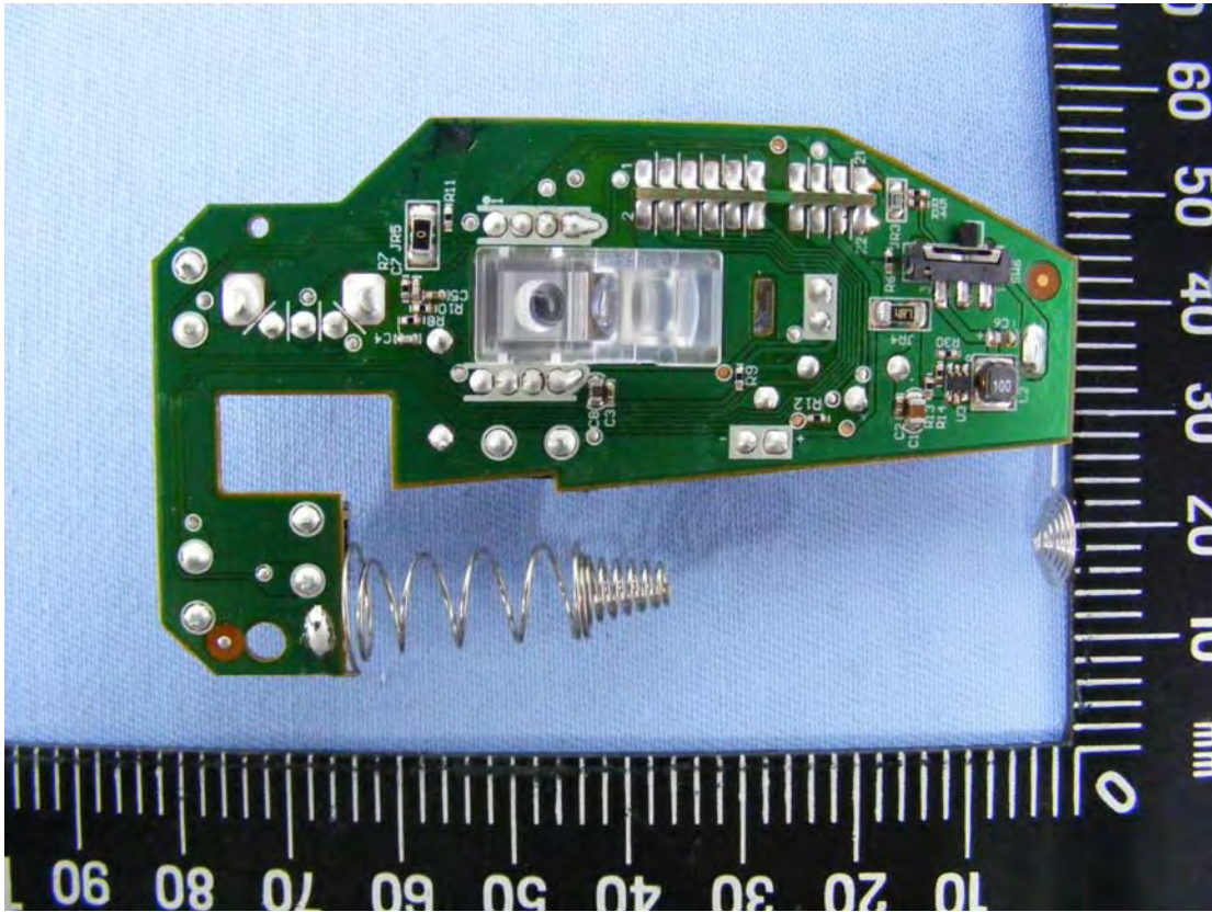
05 Rear view of PCB 1
