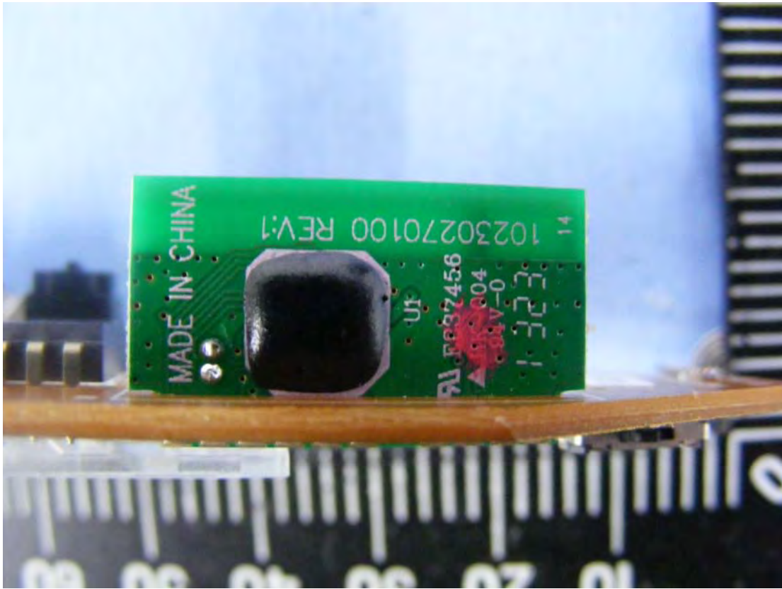
07 Rear view of PCB 2
