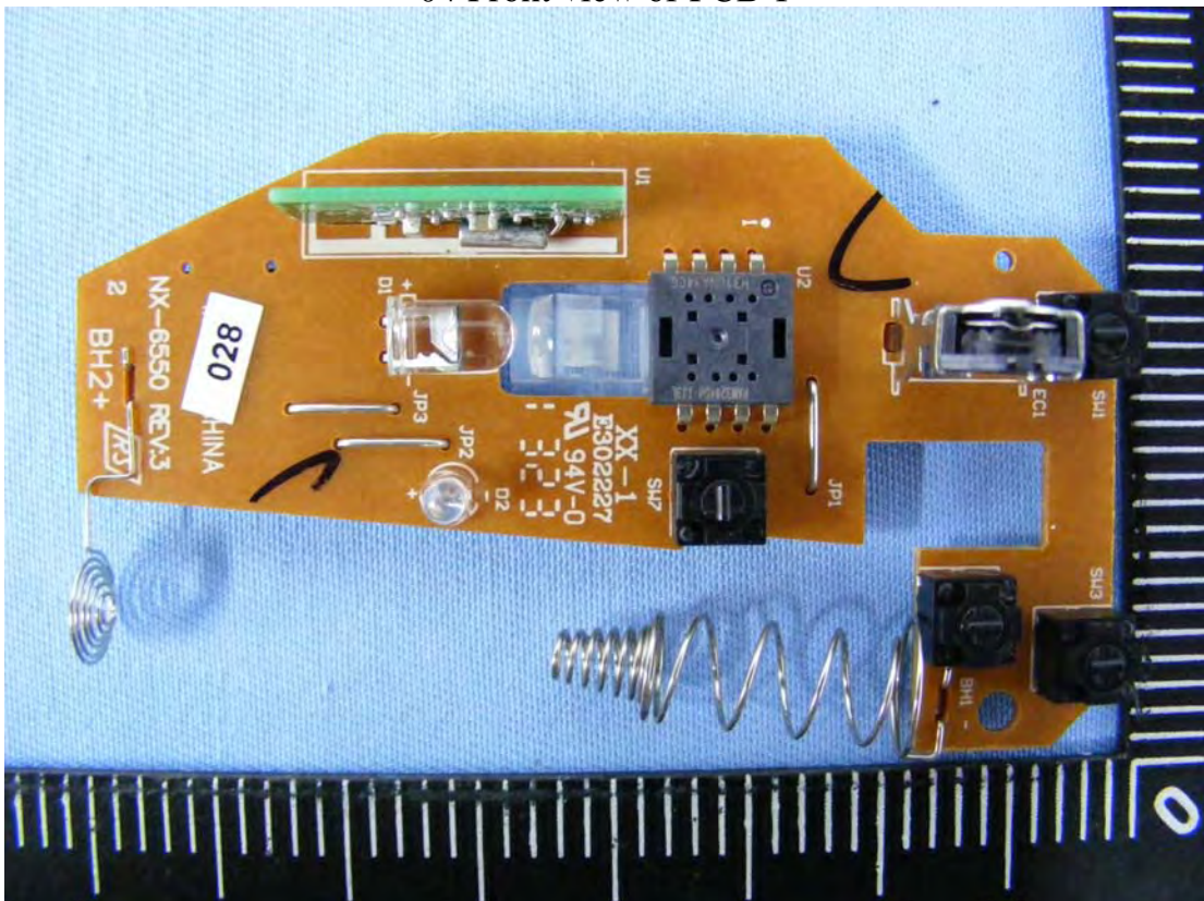
04 Front view of PCB 1
