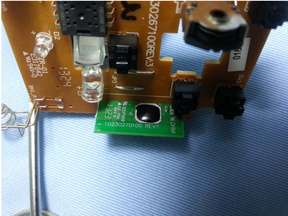
11 Real view of PCB 2
