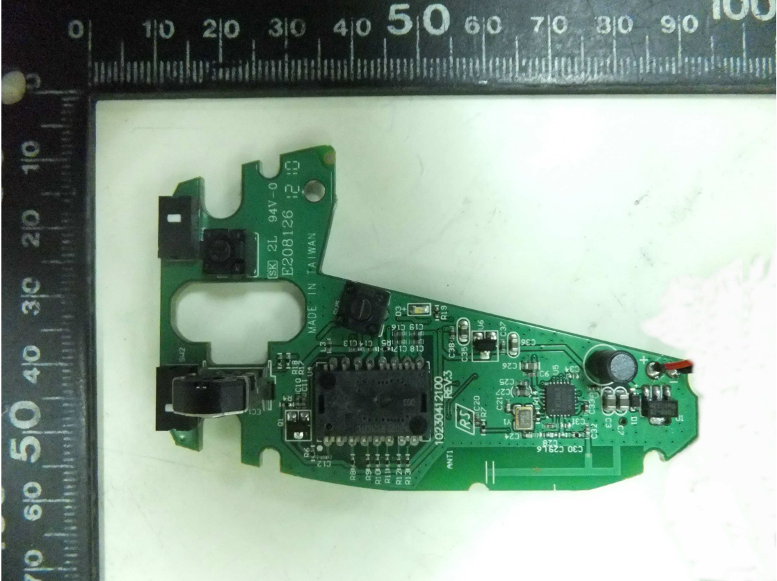
04 Front view of PCB
