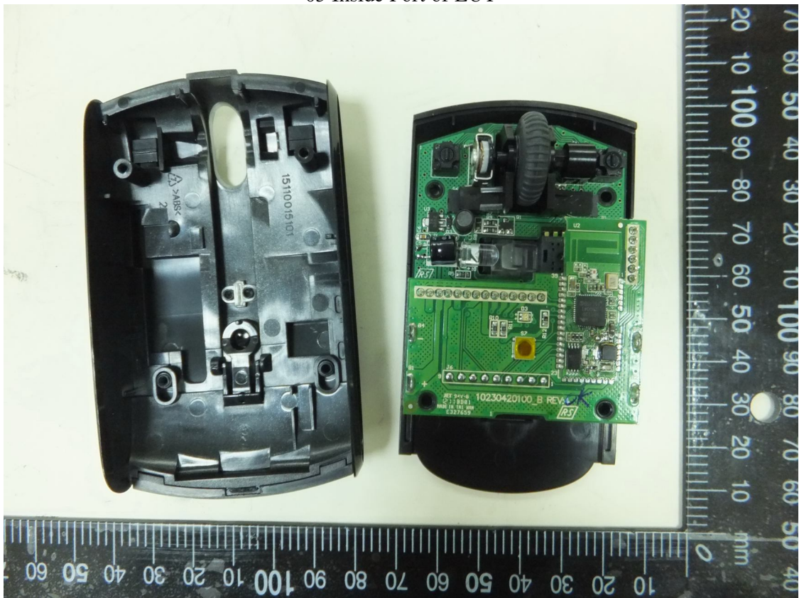
03 Inside Port of EUT
