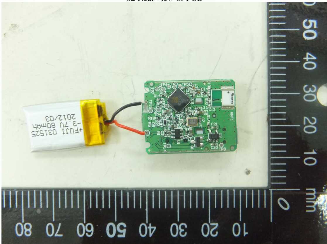
02 Rear view of PCB
