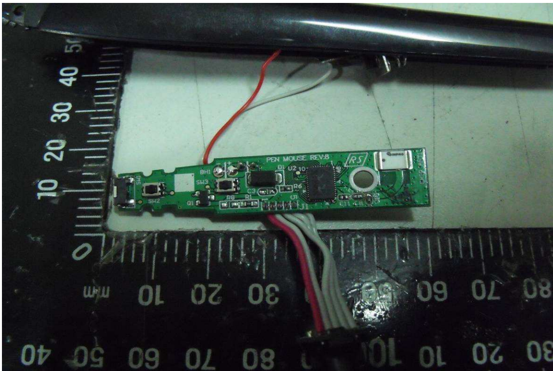
Rear View of Main Board 1
