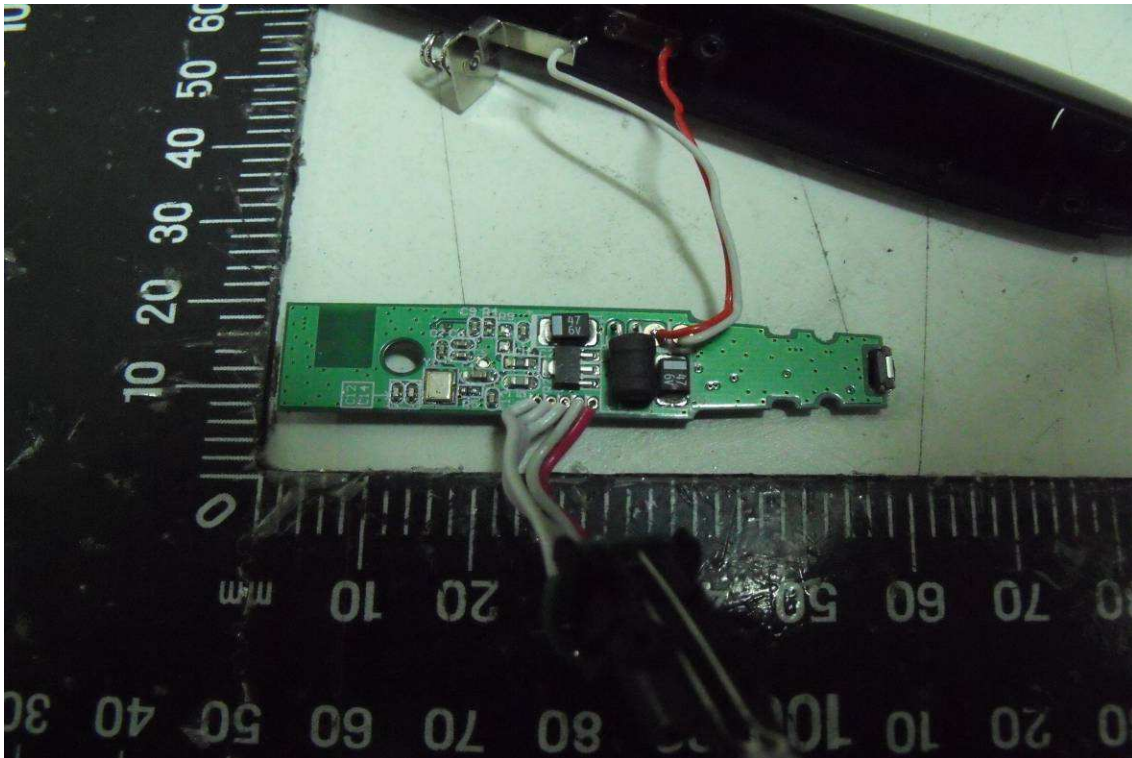
Front View of Main Board 1
