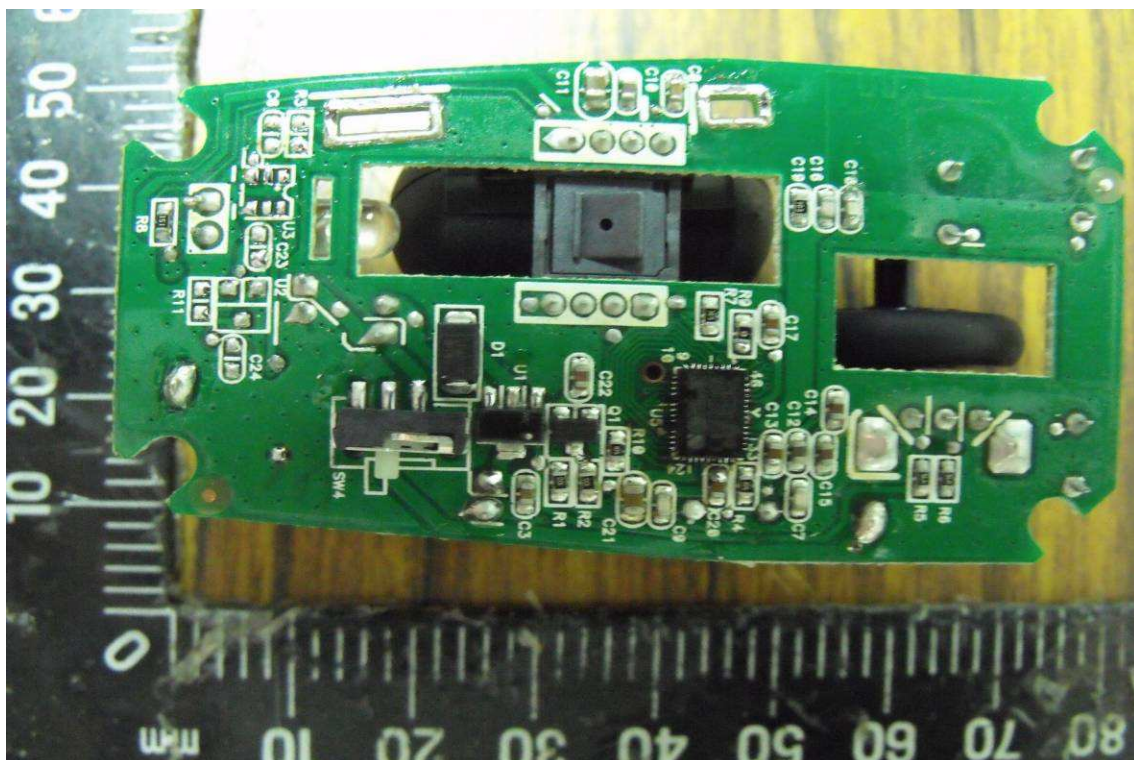
Solder Side of Main Board New EUT
