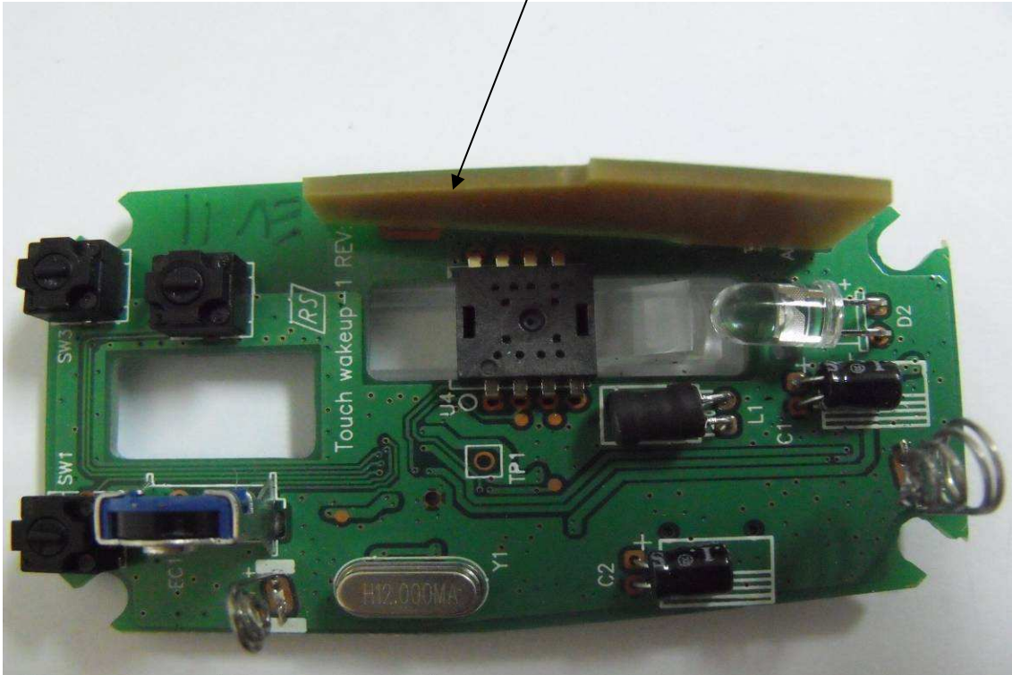
Component Side of Main Board of Old EUT
