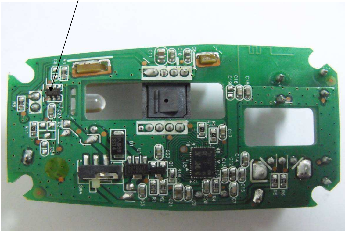
Solder Side of Main Board of Old EUT
