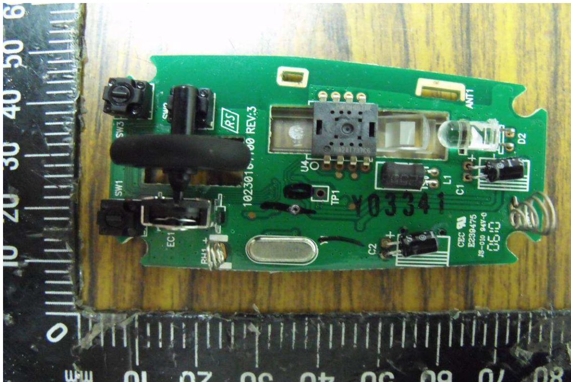
Component Side of Main Board of New EUT
