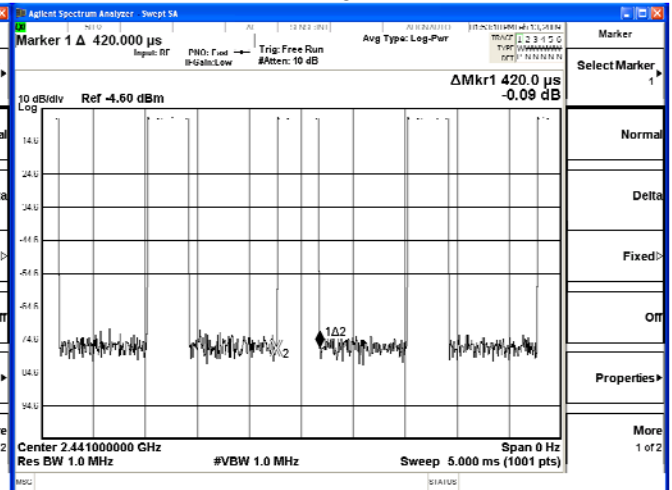
CH 39 Time solt length
