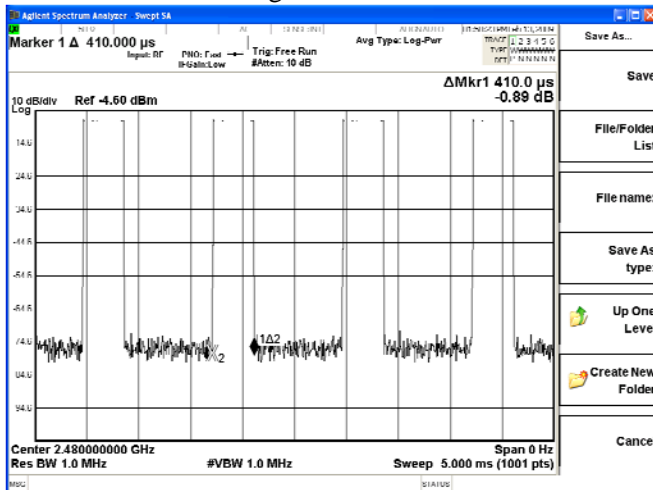
CH 78 T Time solt length
