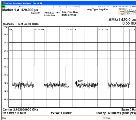
CH 00 Time solt length
