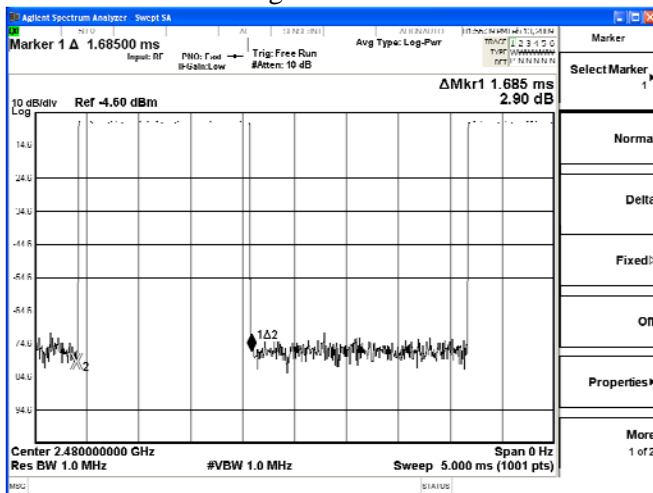
CH 78 T Time slot length
