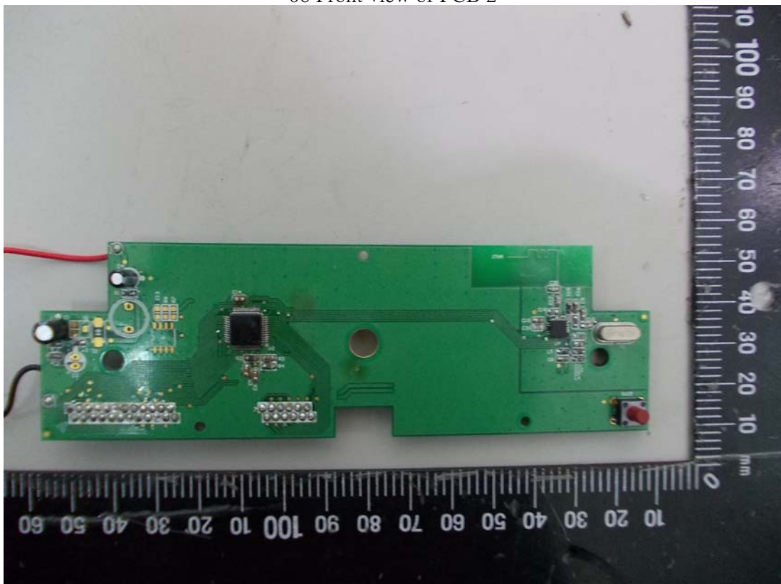
06 Front view of PCB 2
