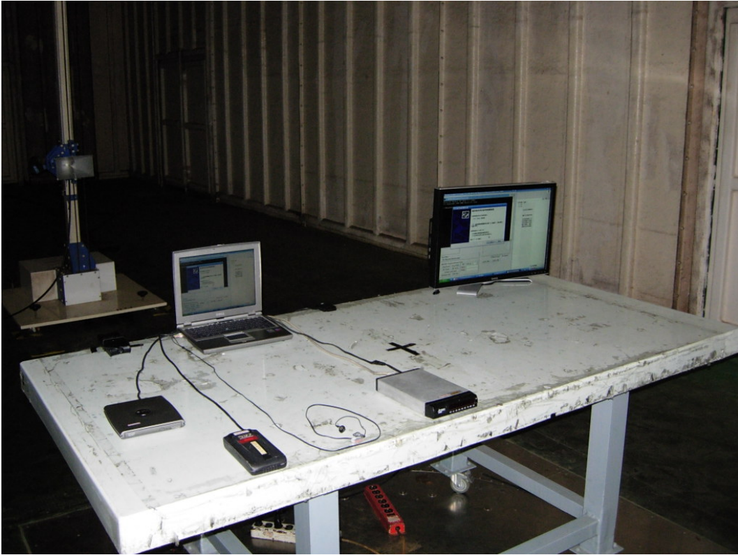
Front View of Radiated Test (Horn antenna)
