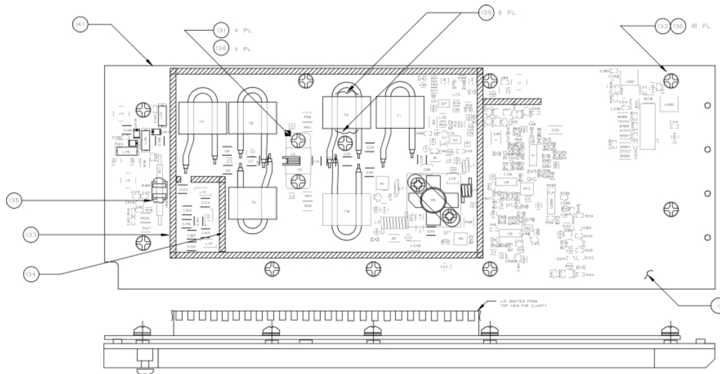
Figure 5-3. VC-401B VC-401B (8.33 kHz) Transmitter/Power Amplifier Module Parts Locator
