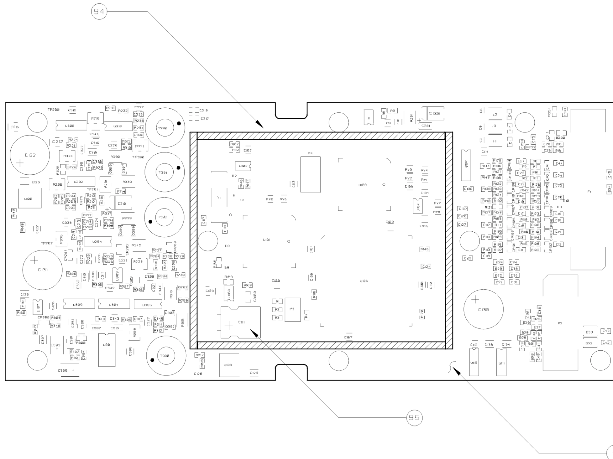
Figure 5-2. VC-401B VC-401B (8.33 kHz) Audio/CPU Module Parts Locator
