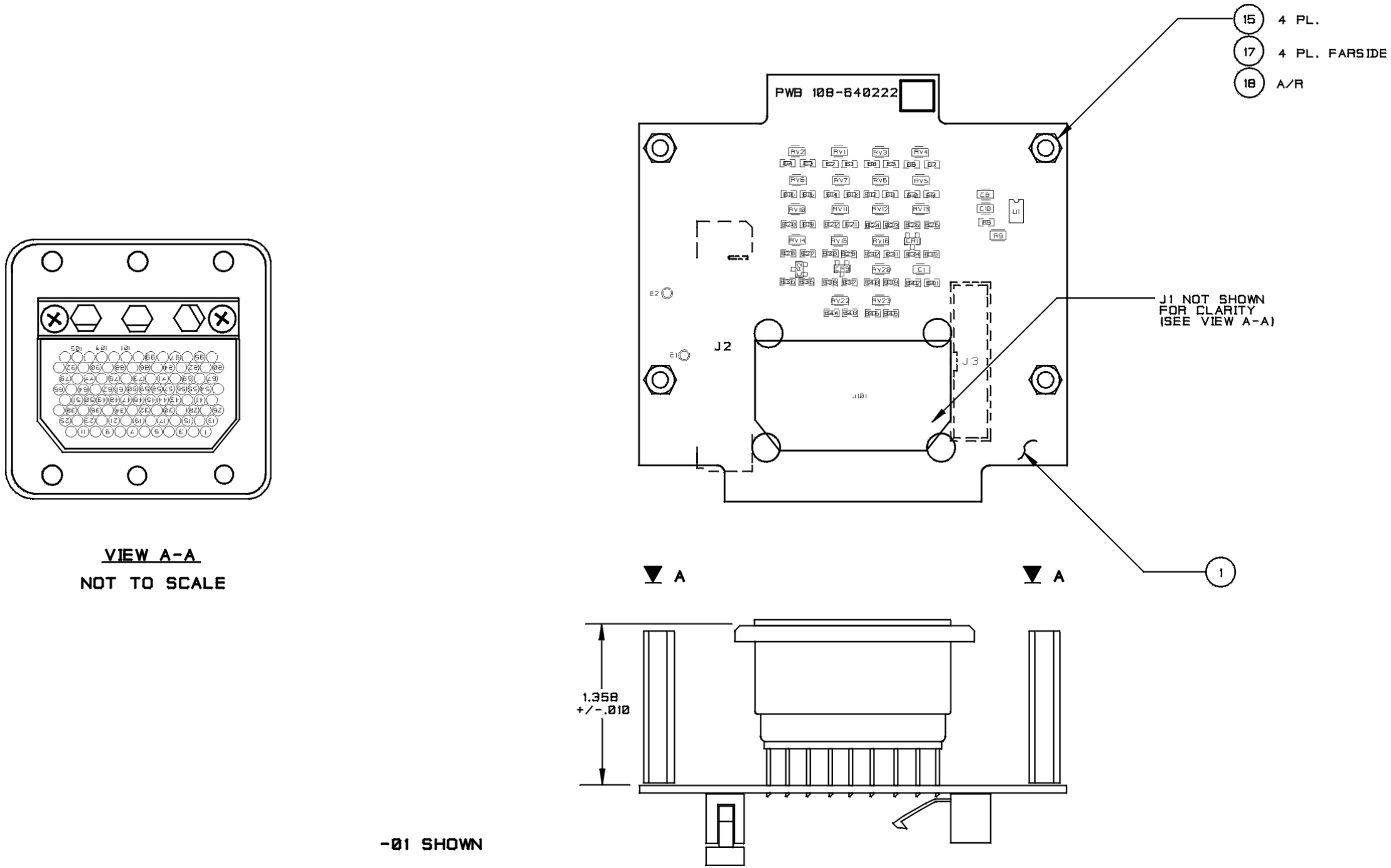
Figure 5-5. VC-401B VC-401B (8.33 kHz) Interconnect Module Parts Locator
