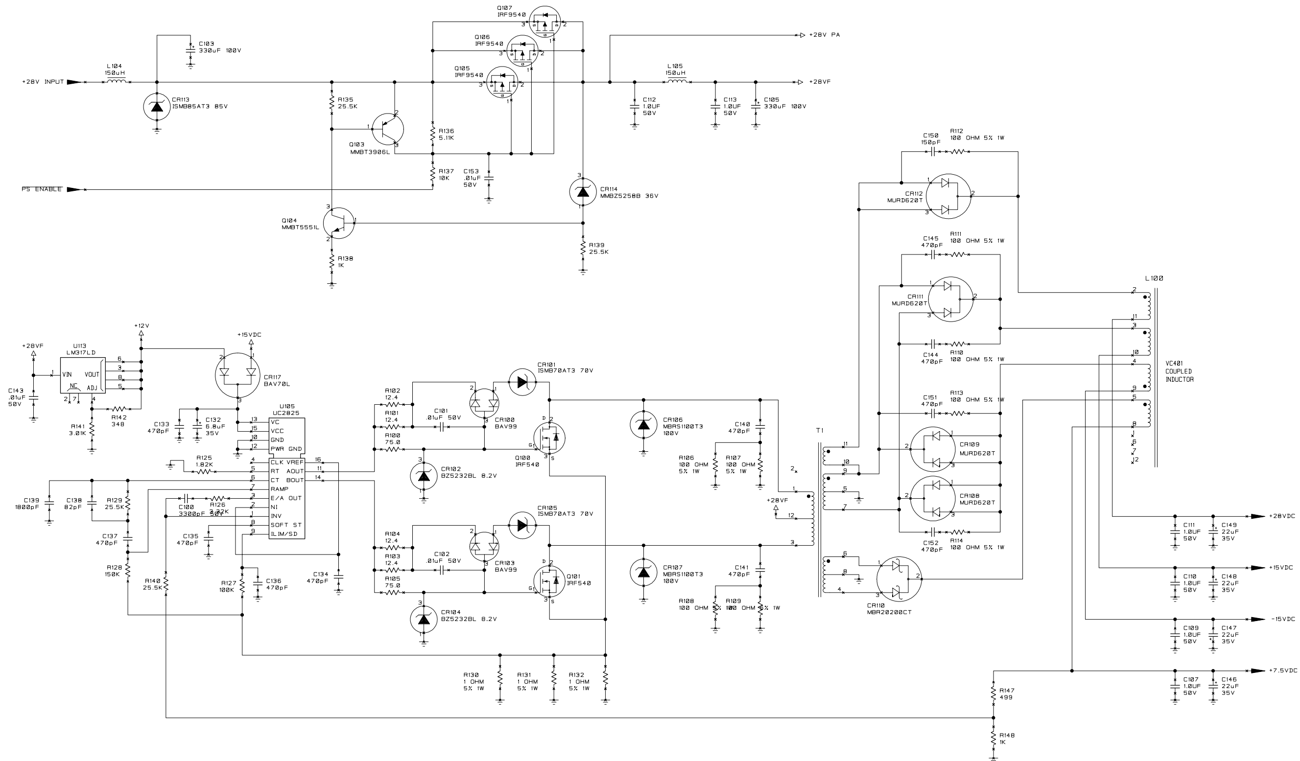
Figure 4-12. VC-401B VHF Communications Transceiver Power Supply Module Schematic Drawing (1 of 2)
