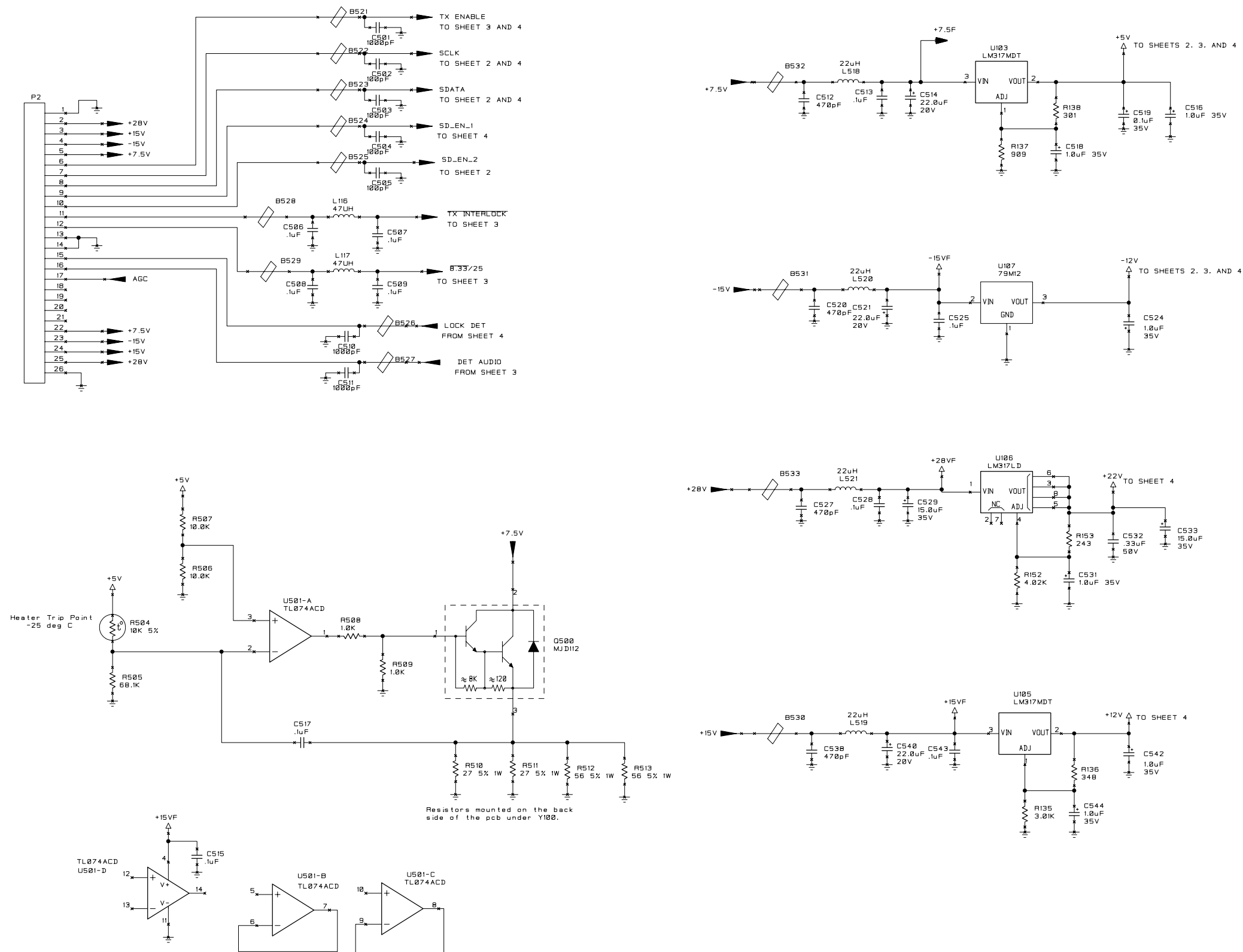
Figure 4-4. VC-401B VHF Communications Transceiver Receiver/Synthesizer Module Schematic Drawing (4 of 4)
