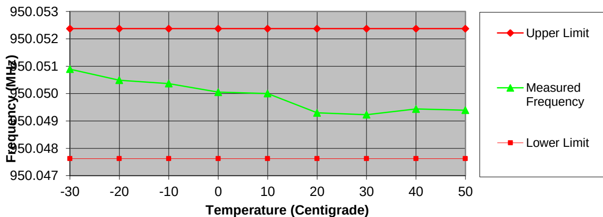
Frequency Stability vs. Temperature
