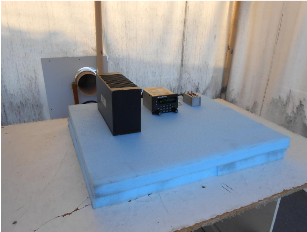
RF Radiated
