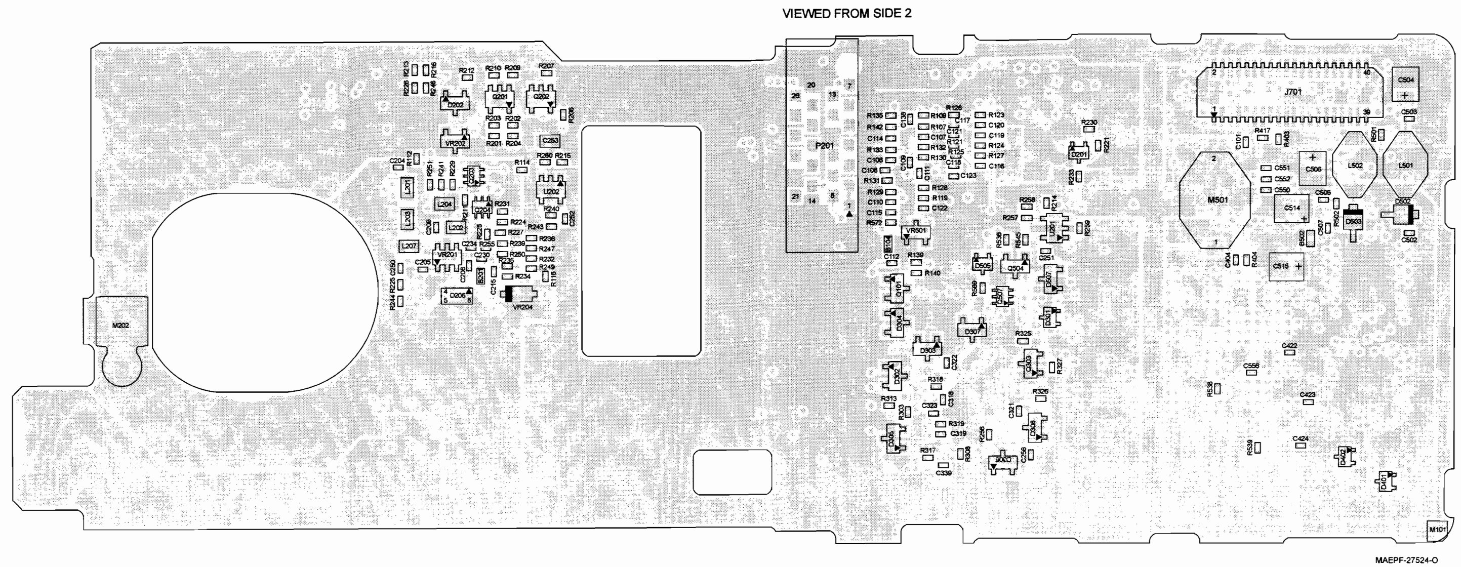
Figure 8-87. NNTN4563A/B VOCON Board Layout—Side 2
