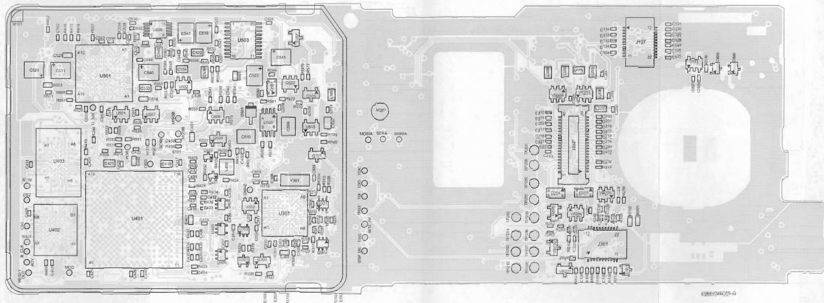
Figure 8-68. NTN9564B VOCON Board Layout—Side 1
