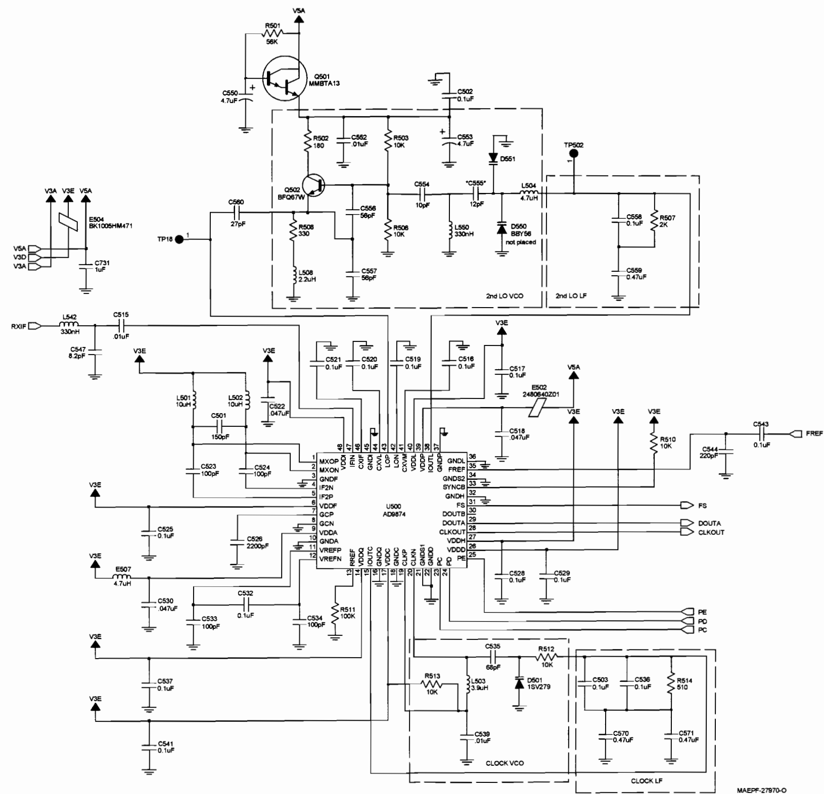
Figure 8-53. NLE 4273A UHF Range 2 Receiver Back End Circuit Schematic
