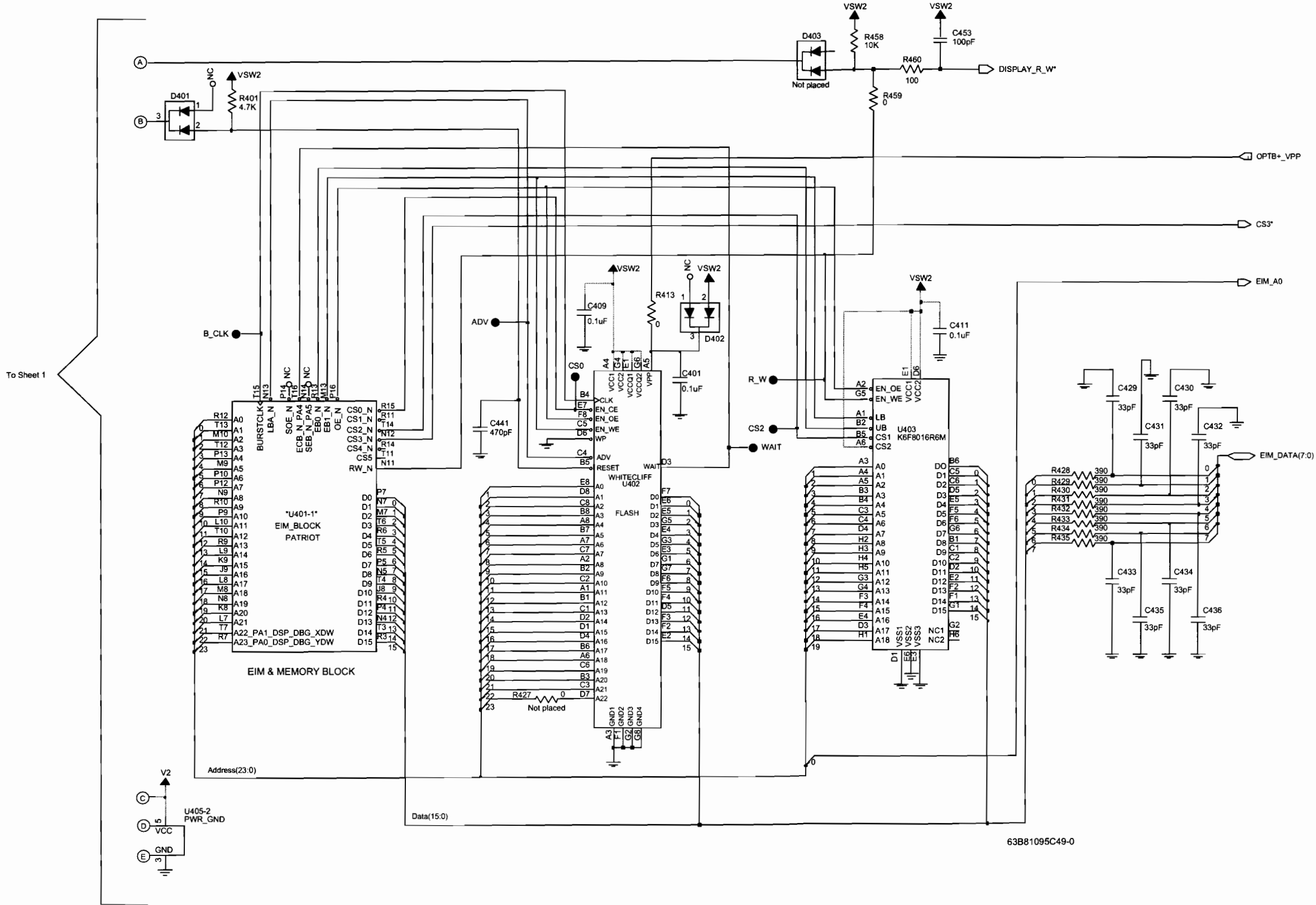
Figure 8-66. NTN9564B VOCON Controller and Memory Circuits—2 of 2
