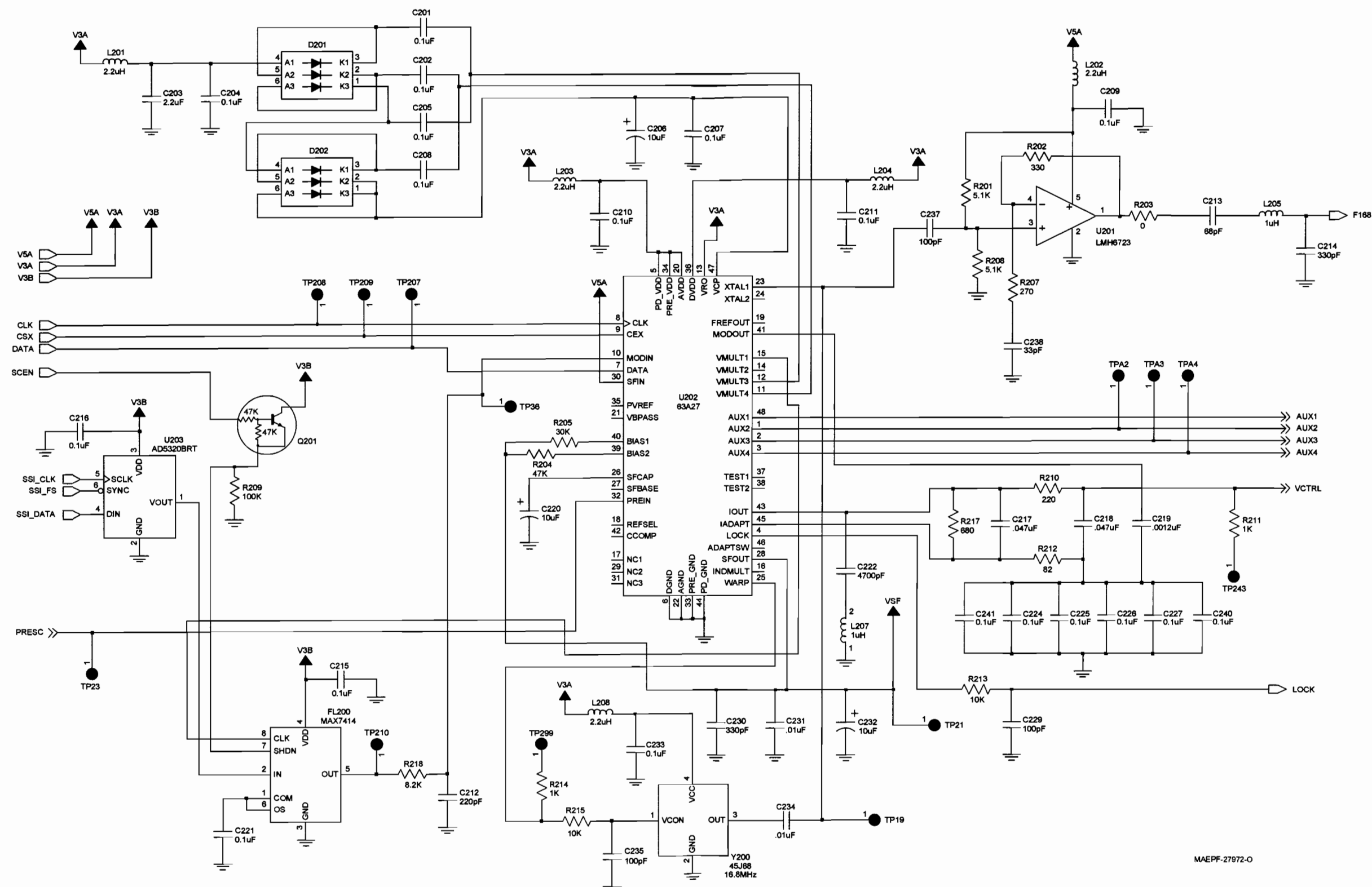
Figure 8-57. NLE 4273A UHF Range 2 Frequency Generation Unit (Synthesizer) Circuit Schematic
