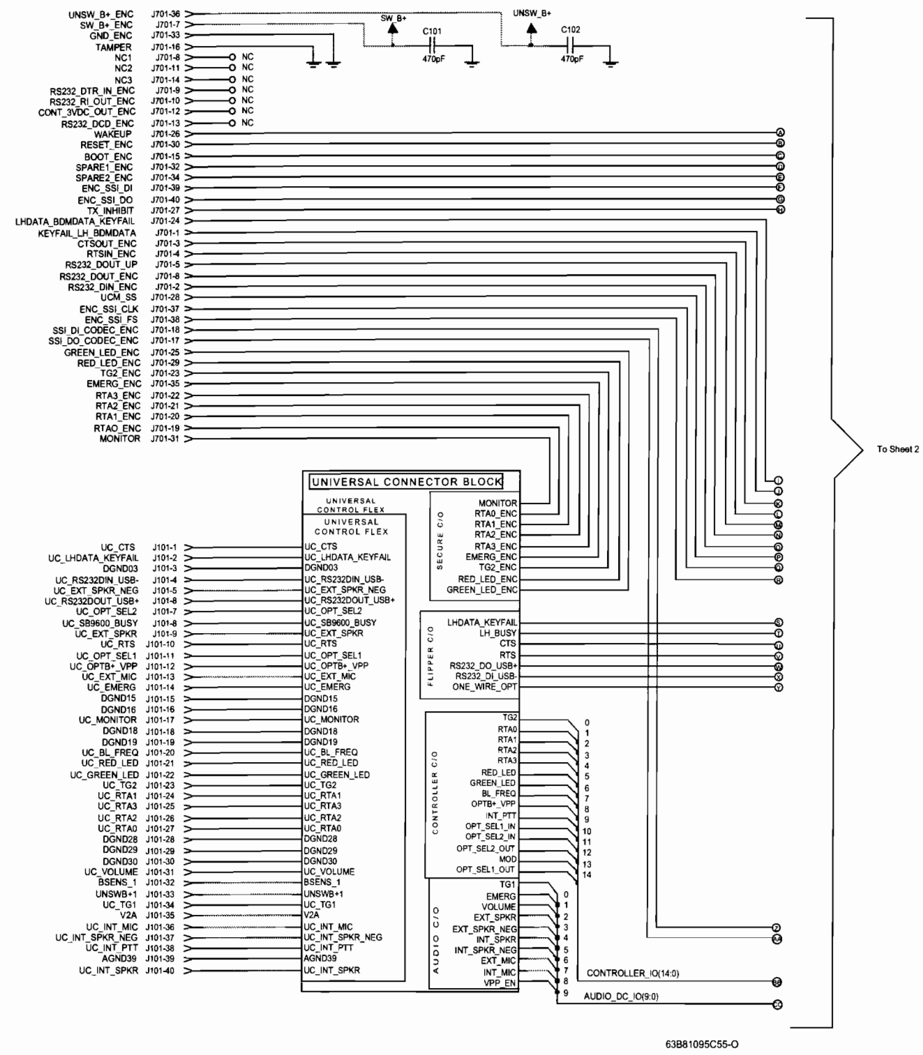
Figure 8-61. NTN9564B VOCON Board Overall Schematic—1 of 2
