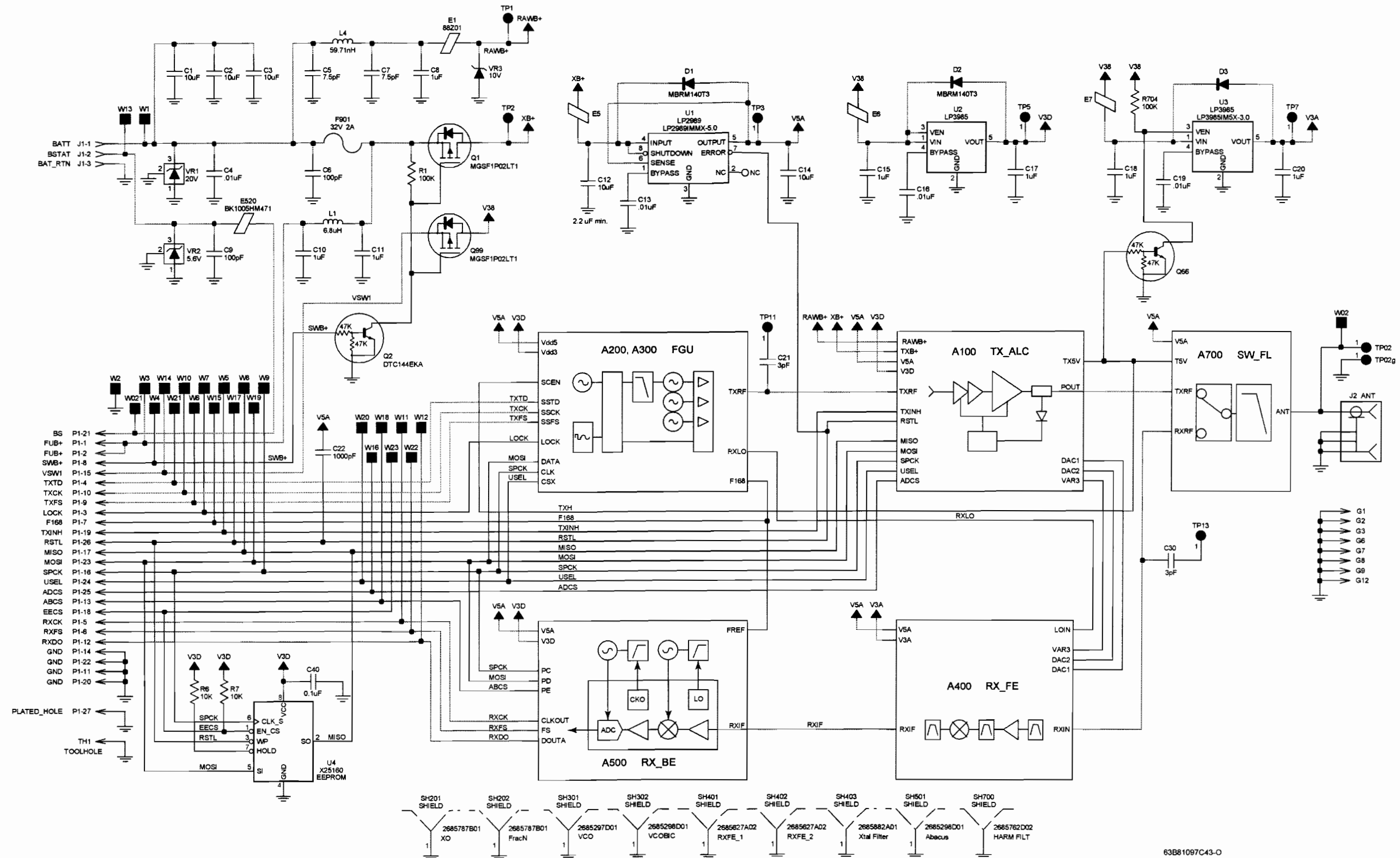
Figure 8-40. NLE4278A UHF Range 1 Transceiver (RF) Board Overall Circuit Schematic
