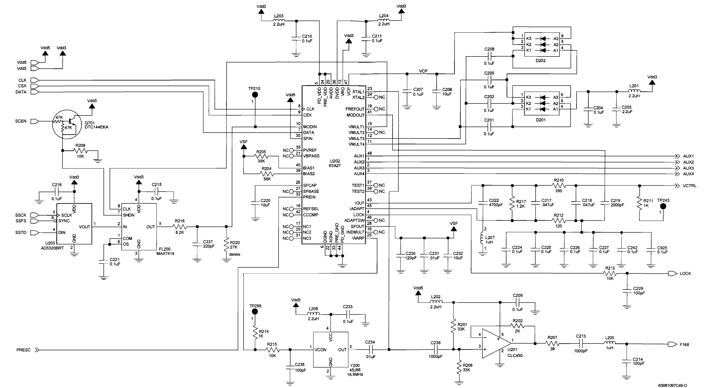
Figure 8-45. NLE4278A UHF Range 1 Frequency Unit (Synthesizer) Circuit
