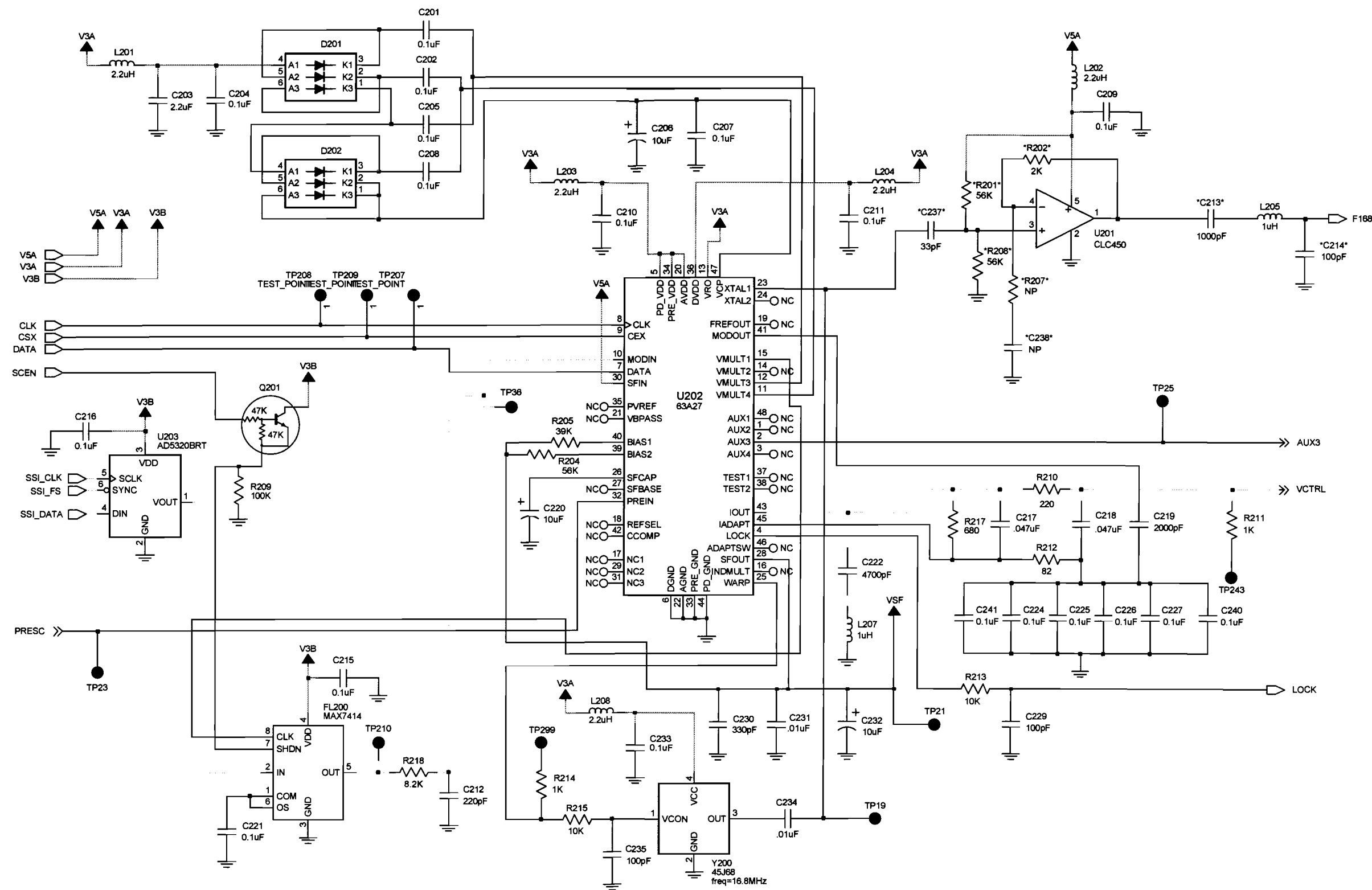
Figure 8-27. NLD8910B VHF Frequency Generation Unit (Synthesizer) Circuit
