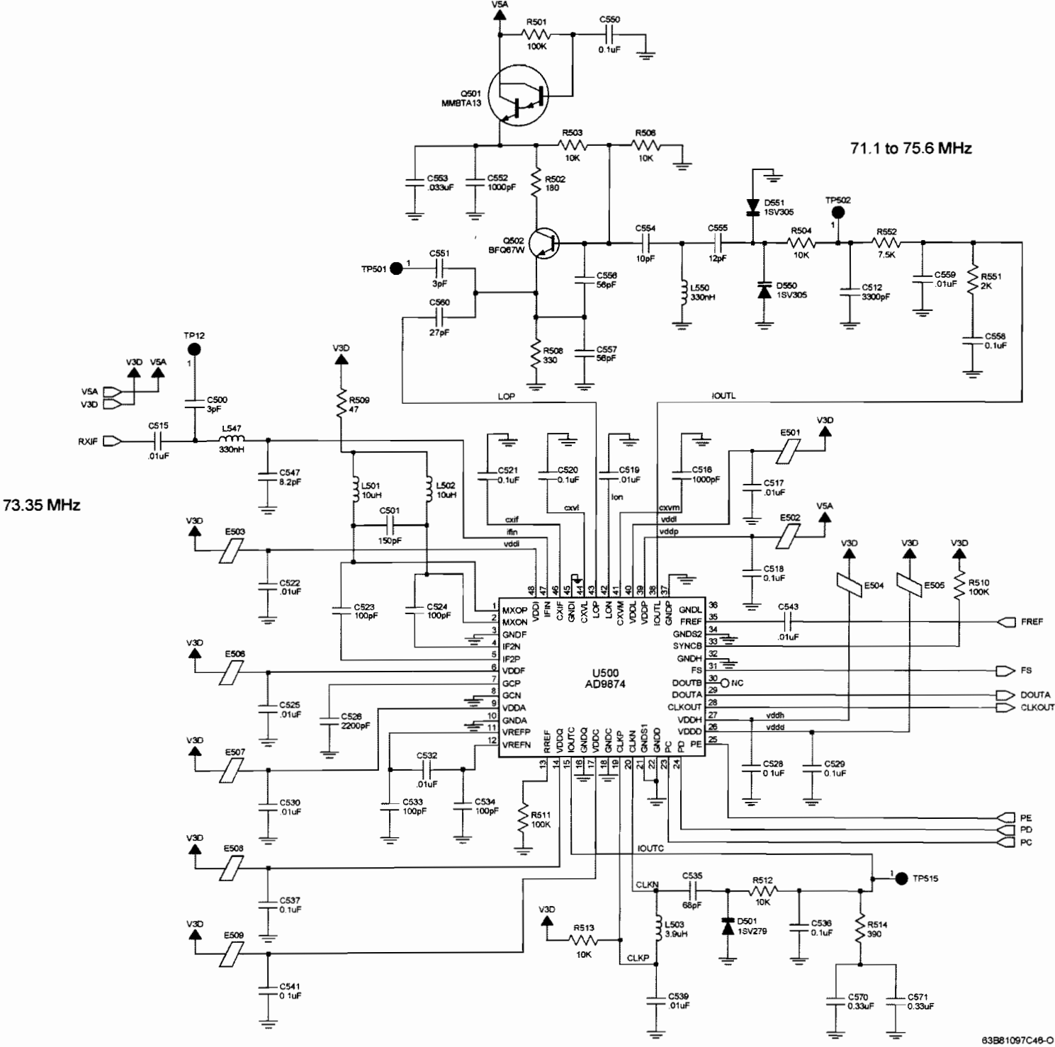
Figure 8-43. NLE4278A UHF Range 1 Receiver Back End Circuit
