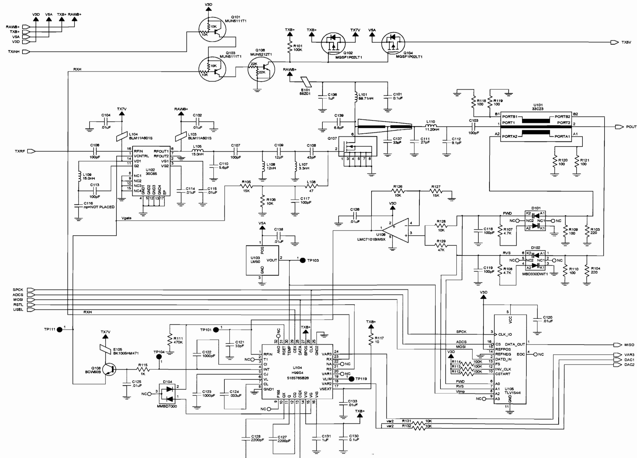
Figure 8-35. NLE4272A UHF Range 1 Transmitter Power Amplifier and Automatic Level Control (TX_ALC) Circuit
