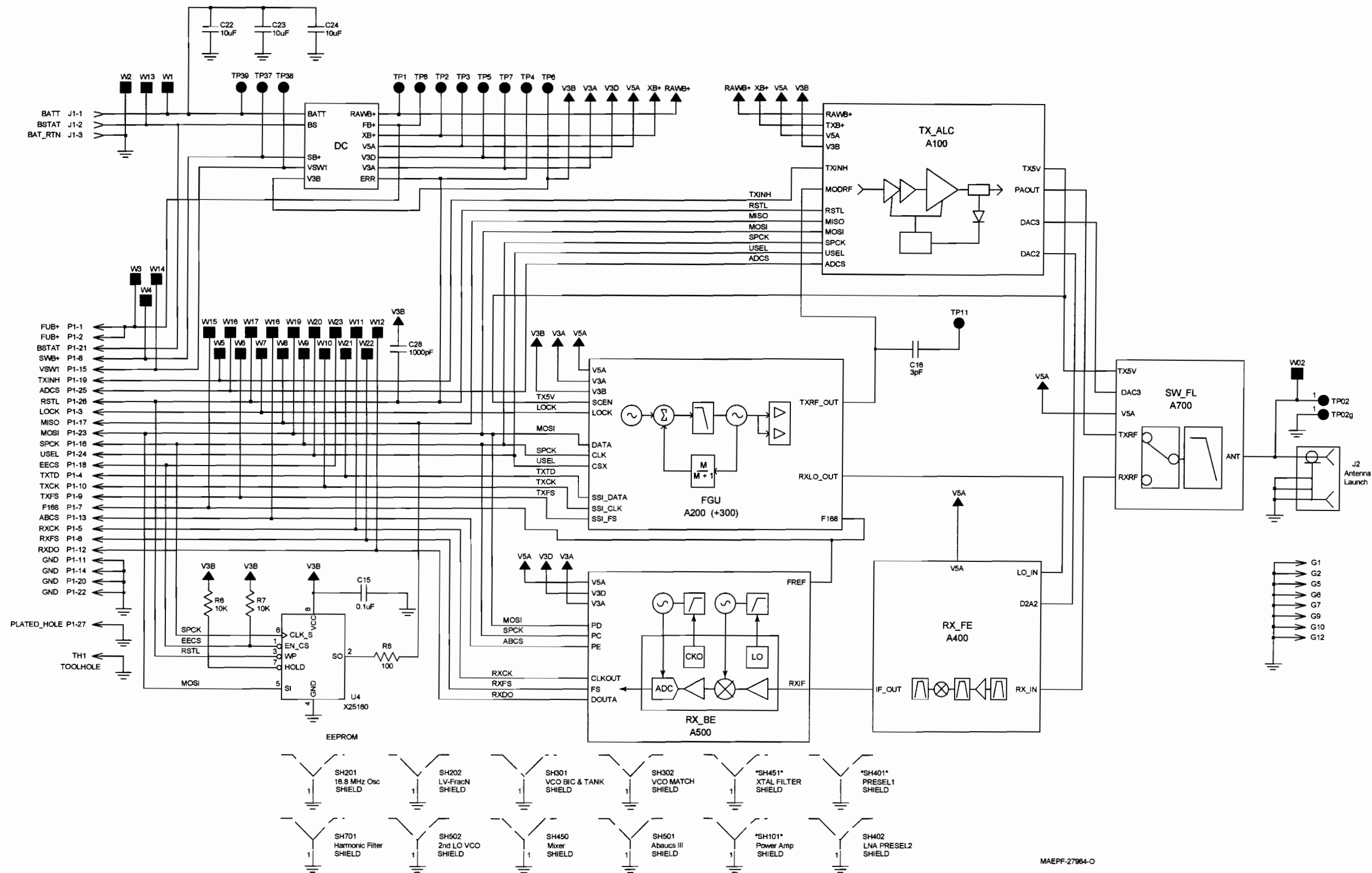
Figure 8-49. NLE 4273A UHF Range 2 Transceiver (RF) Board Overall Circuit Schematic
