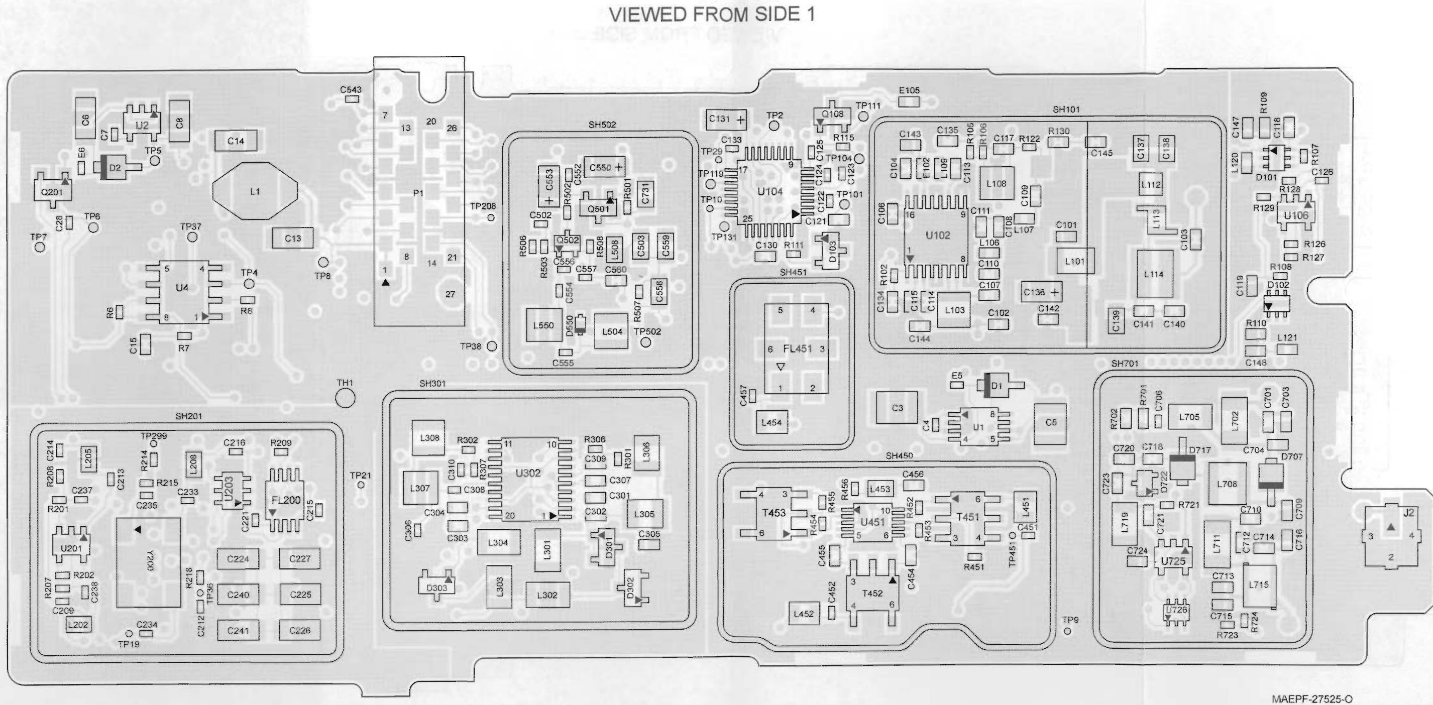
Figure 8-29. NLD8910B VHF Transceiver (RF) Board Layout—Side 1
