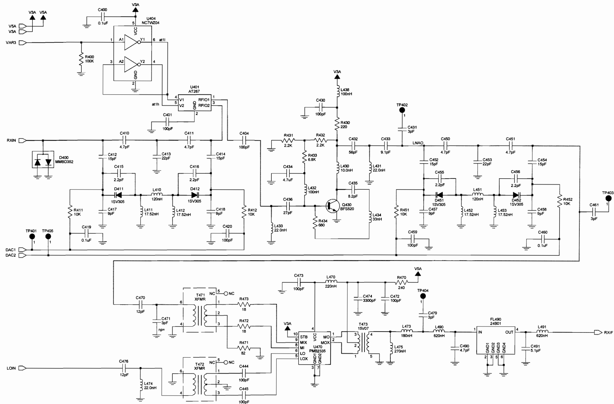
Figure 8-33. NLE4272A UHF Range 1 Receiver Front End (RX_FE) Circuit
