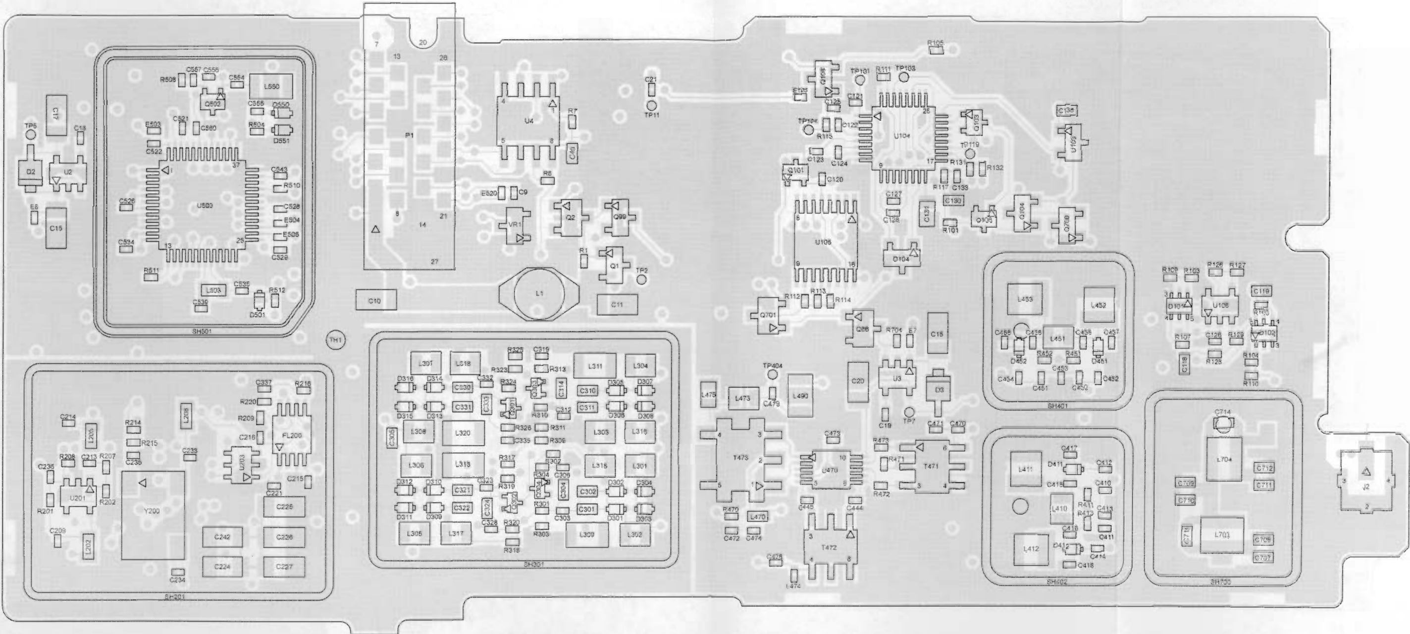
MAEPF-37697-0 Figure 8-38. NLE4272A UHF Range 1 Transceiver (RF) Board Layout—Side 1
