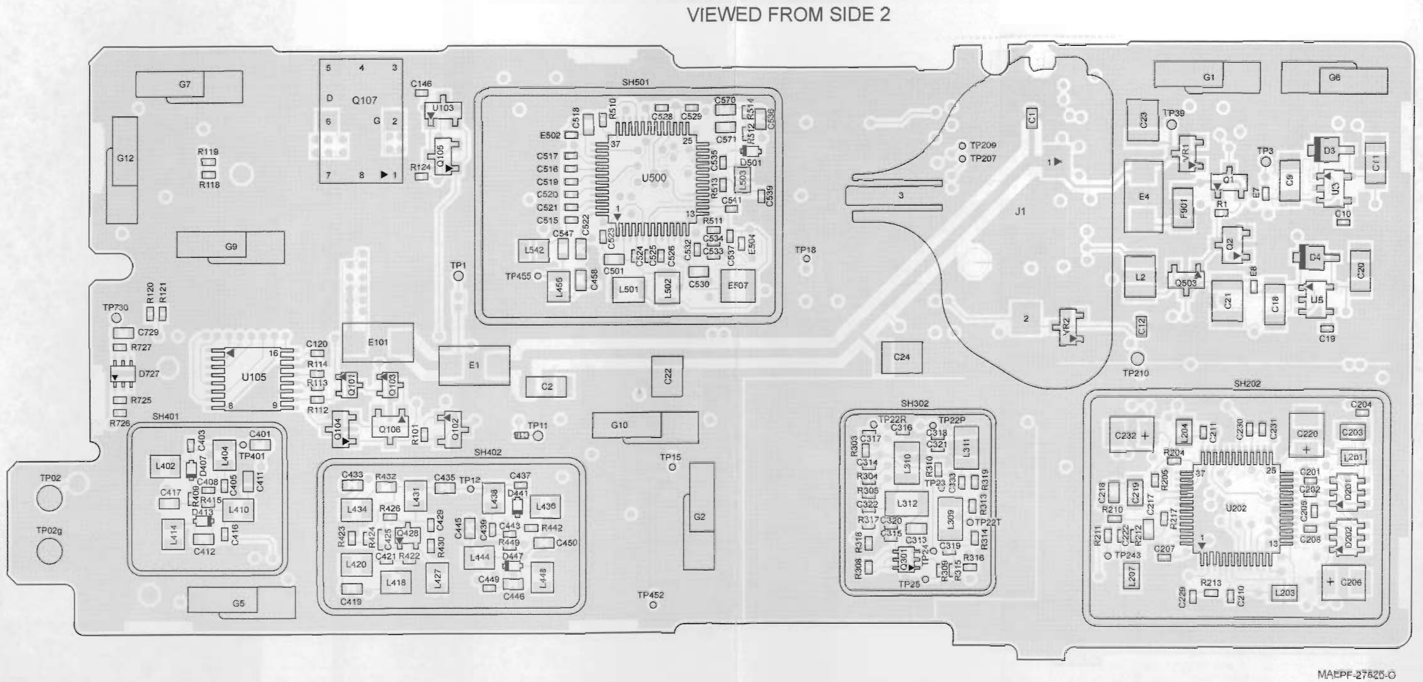
Figure 8-30. NLD8910B VHF Transceiver (RF) Board Layout—Side 2
