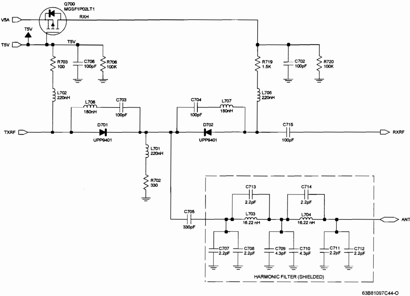
Figure 8-41. NLE4278A UHF Range 1 Antenna Switch and Harmonic Filter Circuits
