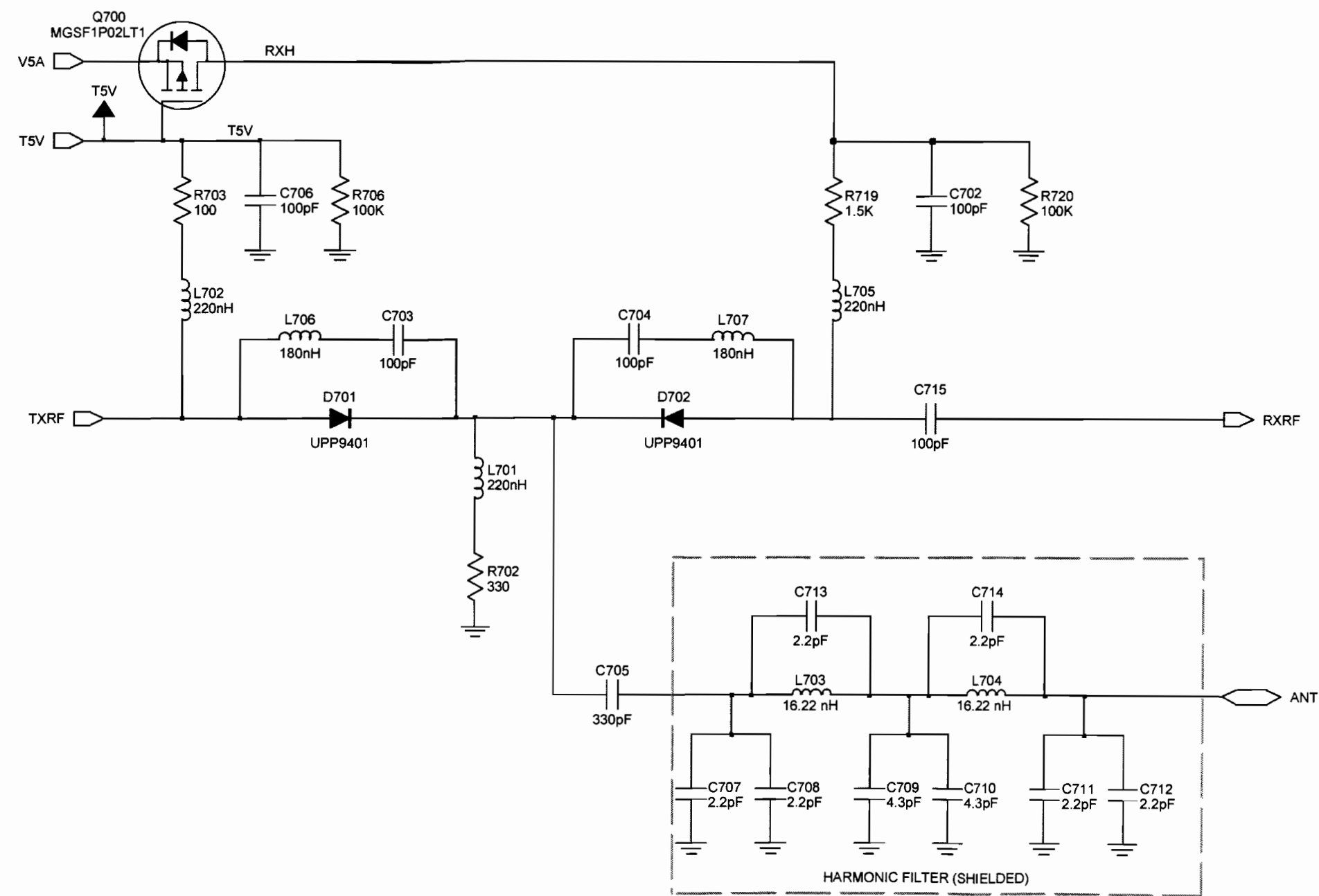
Figure 8-32. NLE4272A UHF Range 1 Antenna Switch and Harmonic Filter Circuits
