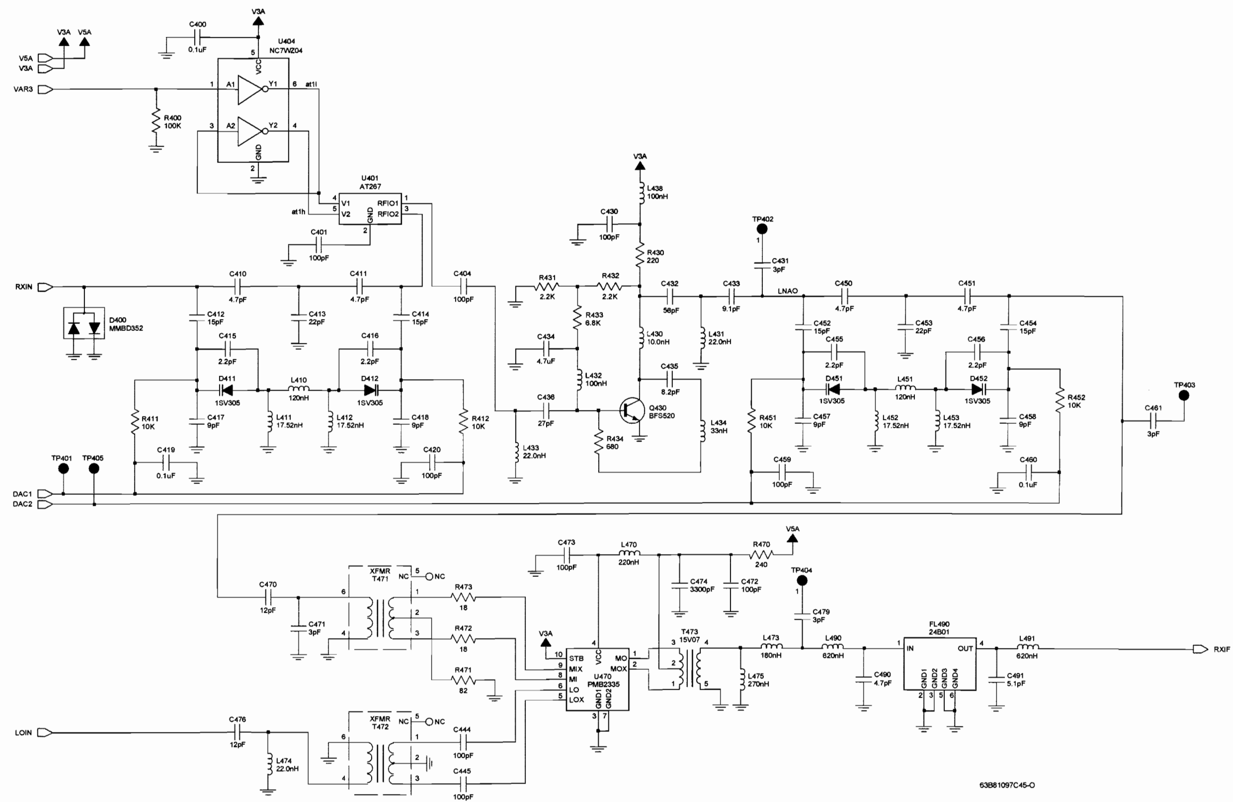
Figure 8-42. NLE4278A UHF Range 1 Receiver Front End Circuit
