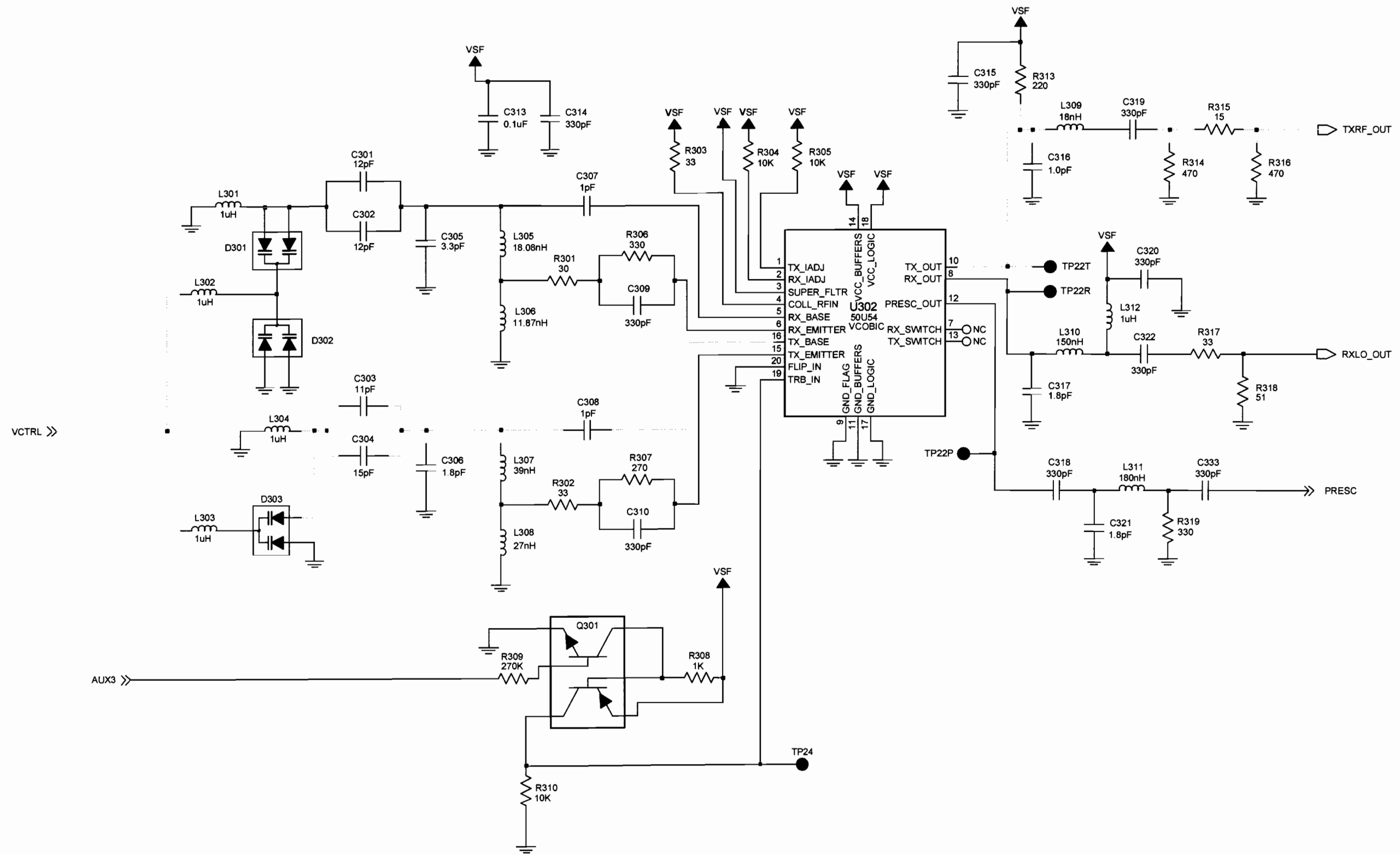
Figure 8-28. NLD8910B VHF Frequency Generation Unit (VCO) Circuit
