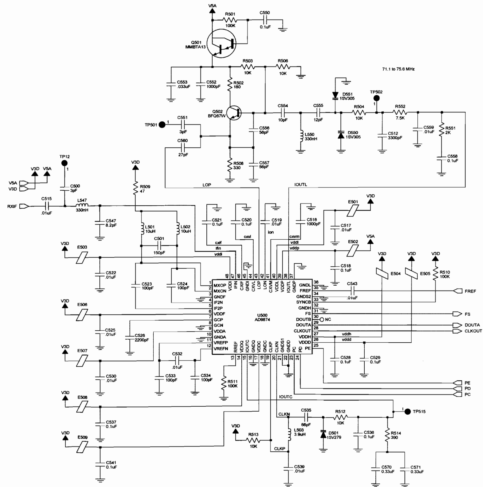
Figure 8-34. NLE4272A UHF Range 1 Receiver Back End (RX_BE) Circuit
