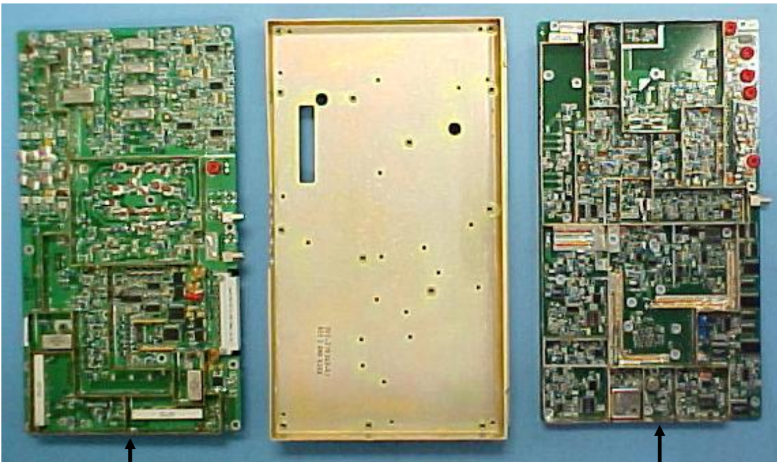
SYNTHESIZER BOARD 300-015471-01
