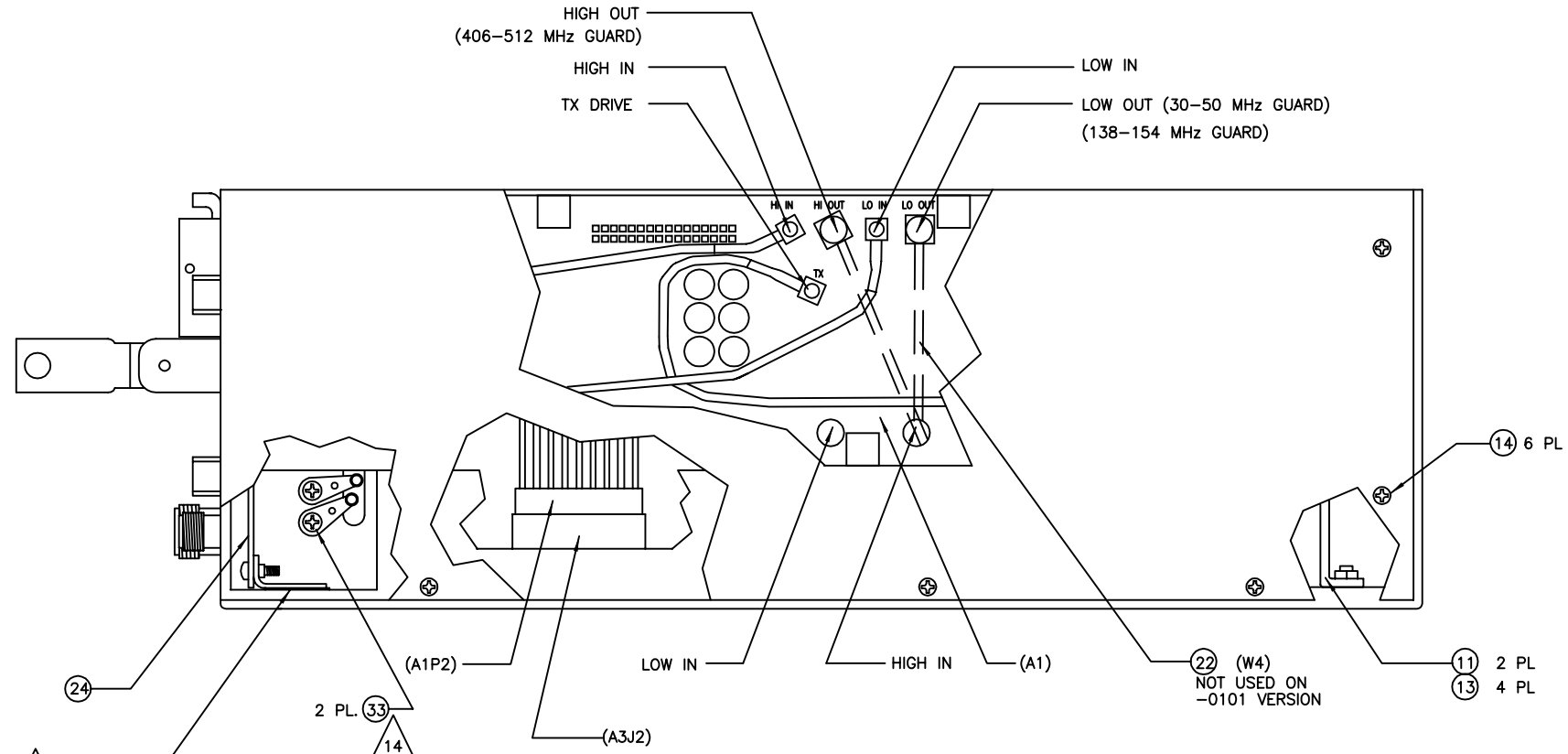
VIEW B-B (-0101 THRU -0401 SHOWN)
