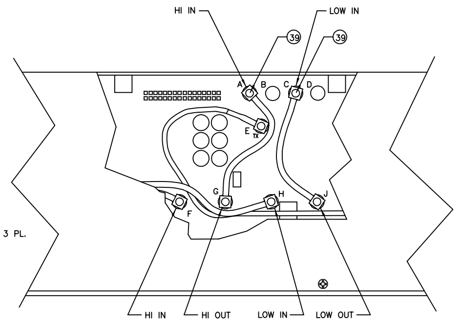
PARTIAL VIEW "F" -1411 THRU -2511 SHOWN
