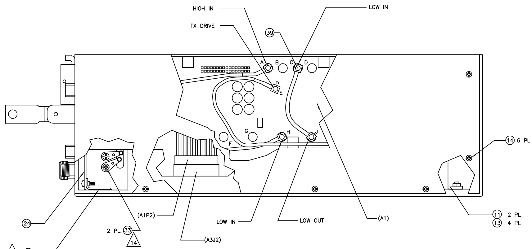
VIEW E-E -0611 THRU -0711
