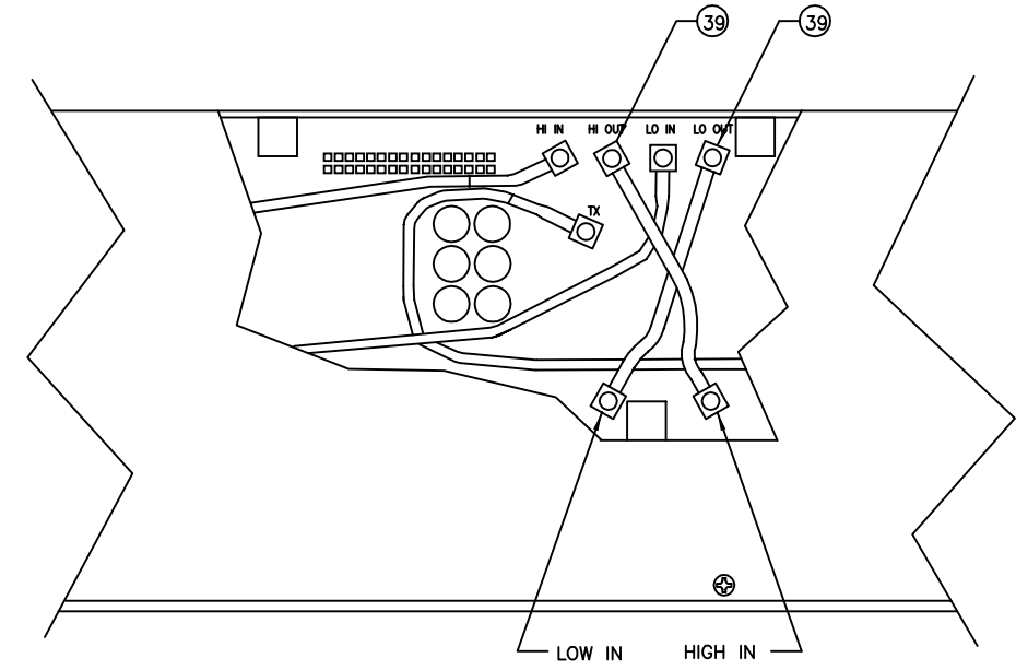
PARTIAL VIEW "C" (-0501 ONLY)
