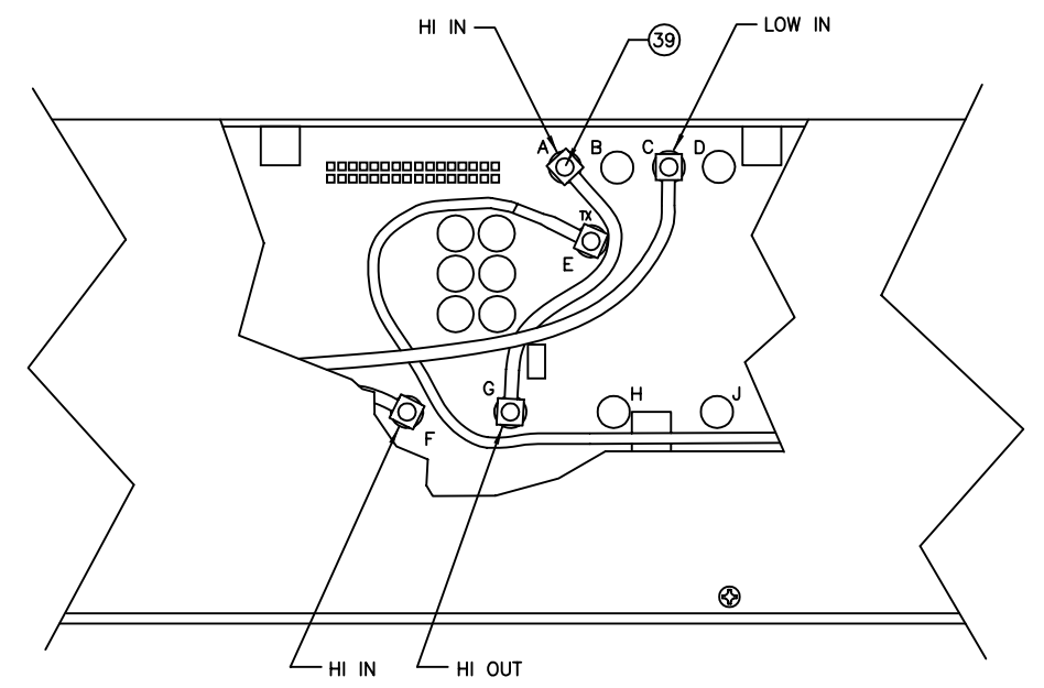
PARTIAL VIEW "F" -0811 THRU -1311 SHOWN
