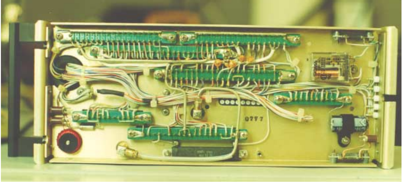
Internal Photos Chassis
